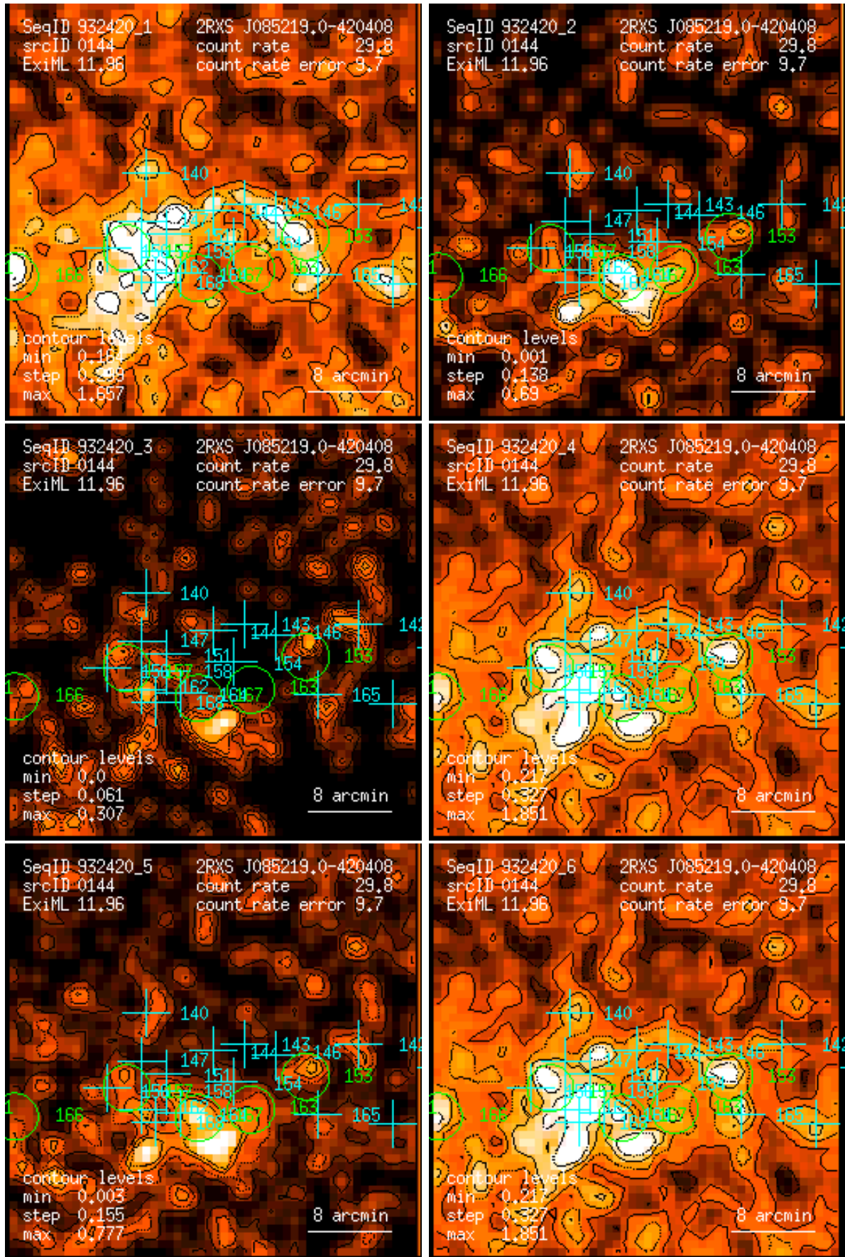
Figure 144: RASS 932420: detection 0144: band rate images, Gaussian filter: (1) PSPC channels 11 – 41, (2) 52 – 90, (3) 91 – 201, (4) 11 – 235, (5) 52 – 201, (6) 11 – 201. Broad band rates in counts/ks. Band rate contour levels in counts/ks/arcmin 2 .
