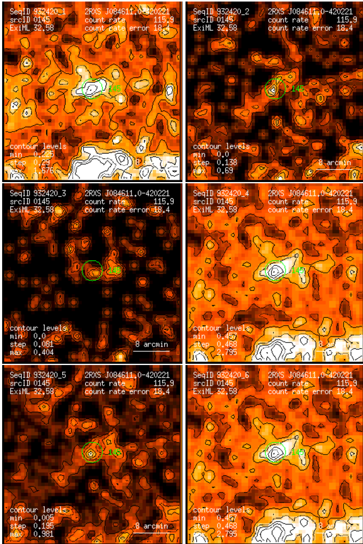
Figure 145: RASS 932420: detection 0145: band rate images, Gaussian filter: (1) PSPC channels 11 – 41, (2) 52 – 90, (3) 91 – 201, (4) 11 – 235, (5) 52 – 201, (6) 11 – 201. Broad band rates in counts/ks. Band rate contour levels in counts/ks/arcmin 2 .
