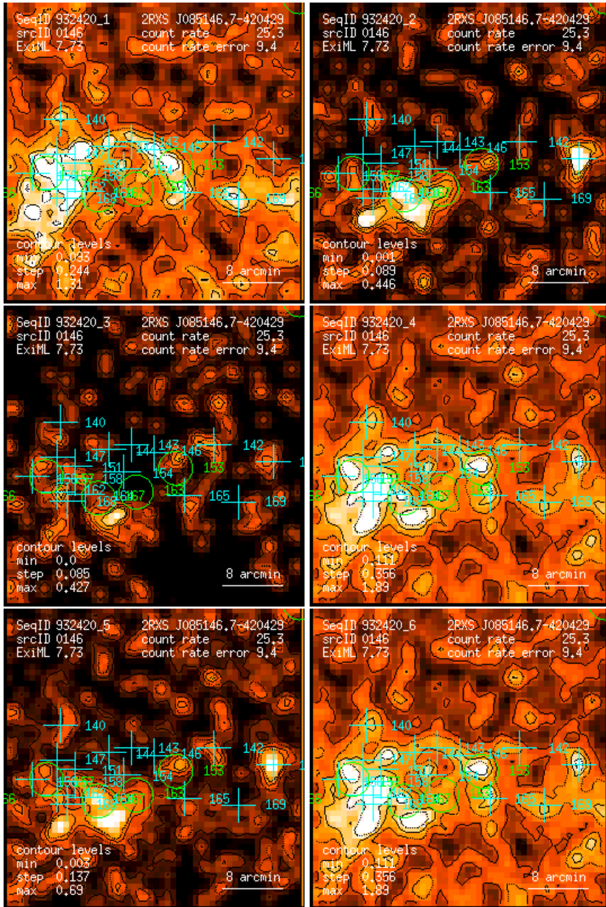
Figure 146: RASS 932420: detection 0146: band rate images, Gaussian filter: (1) PSPC channels 11 – 41, (2) 52 – 90, (3) 91 – 201, (4) 11 – 235, (5) 52 – 201, (6) 11 – 201. Broad band rates in counts/ks. Band rate contour levels in counts/ks/arcmin 2 .
