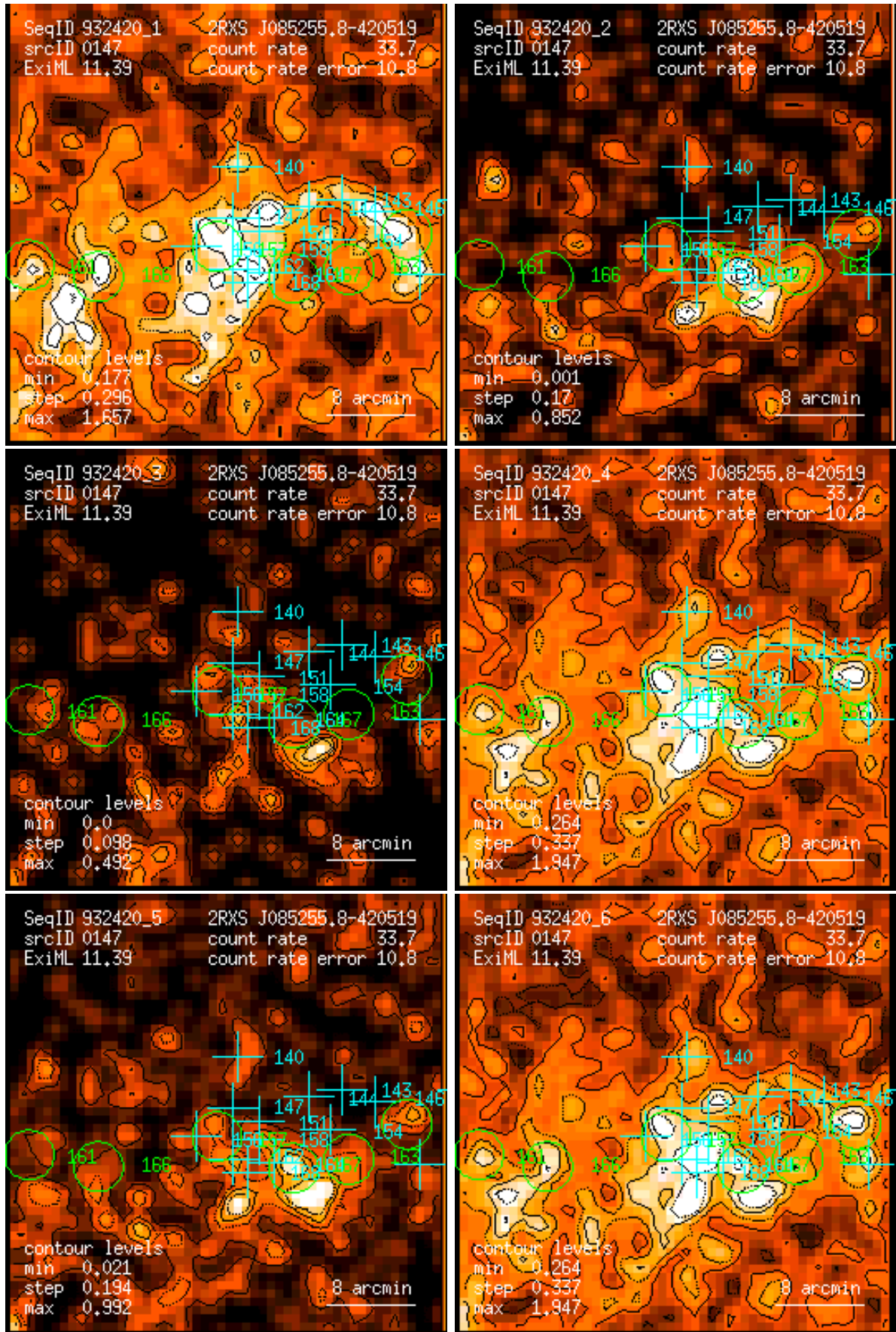
Figure 147: RASS 932420: detection 0147: band rate images, Gaussian filter: (1) PSPC channels 11 – 41, (2) 52 – 90, (3) 91 – 201, (4) 11 – 235, (5) 52 – 201, (6) 11 – 201. Broad band rates in counts/ks. Band rate contour levels in counts/ks/arcmin 2 .
