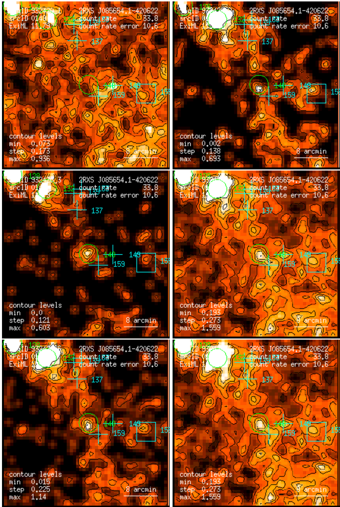
Figure 148: RASS 932420: detection 0148: band rate images, Gaussian filter: (1) PSPC channels 11 – 41, (2) 52 – 90, (3) 91 – 201, (4) 11 – 235, (5) 52 – 201, (6) 11 – 201. Broad band rates in counts/ks. Band rate contour levels in counts/ks/arcmin 2 .
