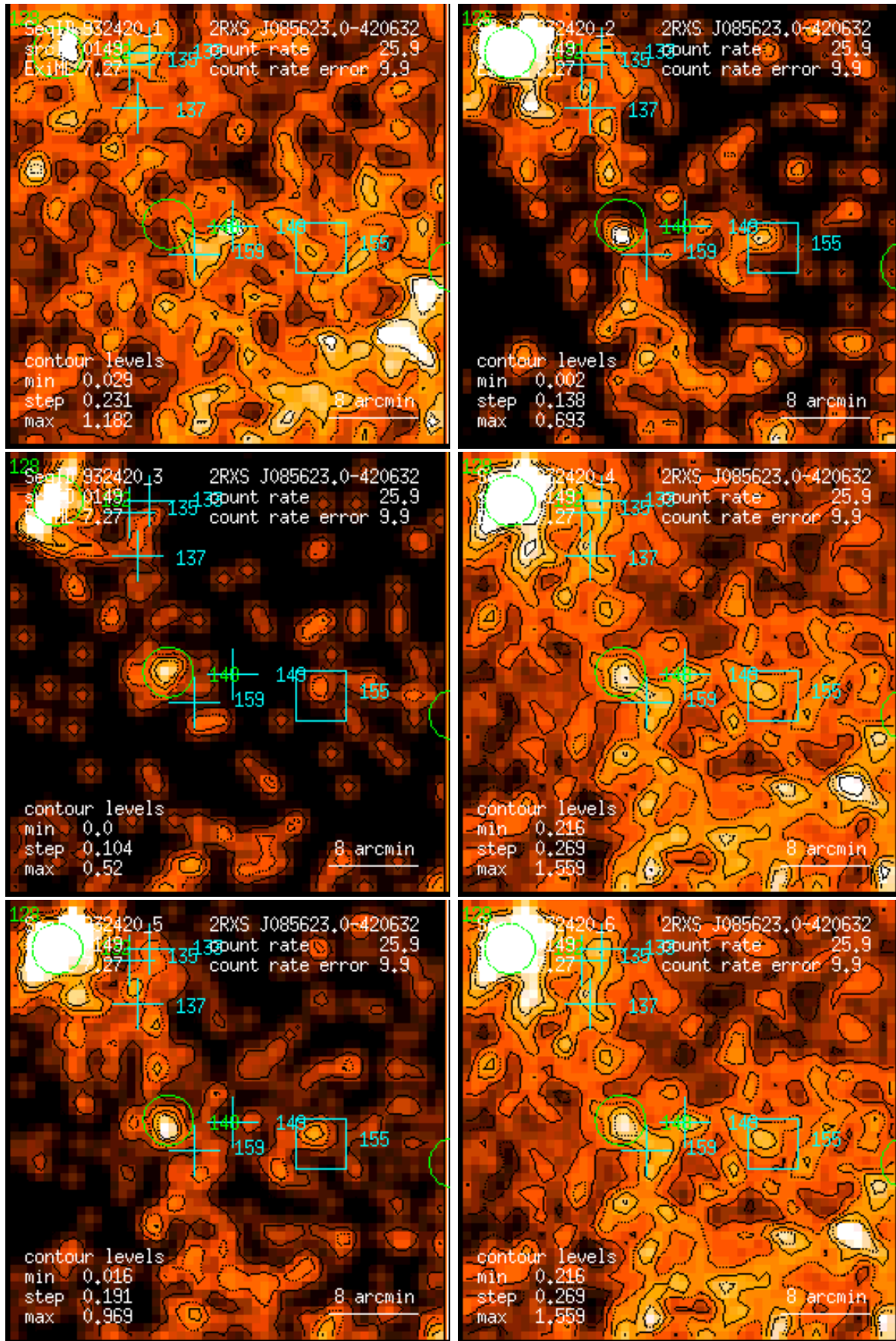
Figure 149: RASS 932420: detection 0149: band rate images, Gaussian filter: (1) PSPC channels 11 – 41, (2) 52 – 90, (3) 91 – 201, (4) 11 – 235, (5) 52 – 201, (6) 11 – 201. Broad band rates in counts/ks. Band rate contour levels in counts/ks/arcmin 2 .
