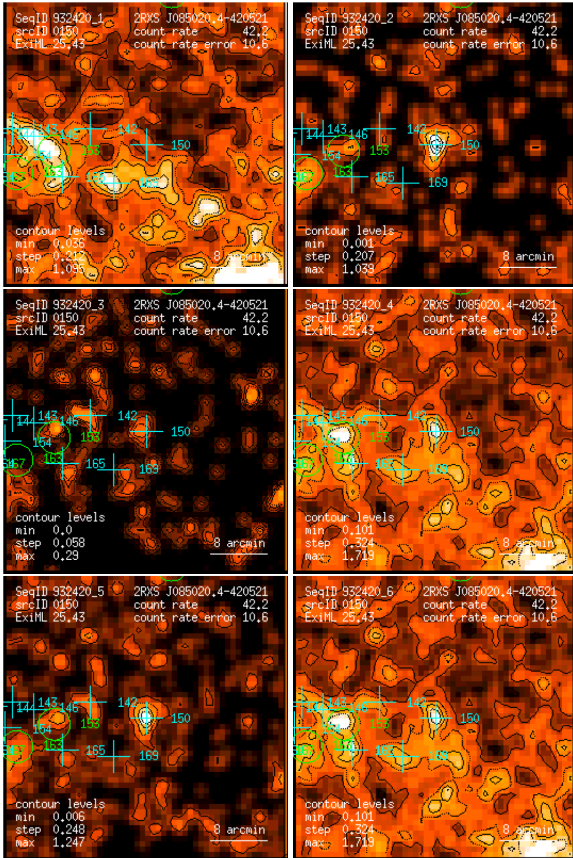
Figure 150: RASS 932420: detection 0150: band rate images, Gaussian filter: (1) PSPC channels 11 – 41, (2) 52 – 90, (3) 91 – 201, (4) 11 – 235, (5) 52 – 201, (6) 11 – 201. Broad band rates in counts/ks. Band rate contour levels in counts/ks/arcmin 2 .
