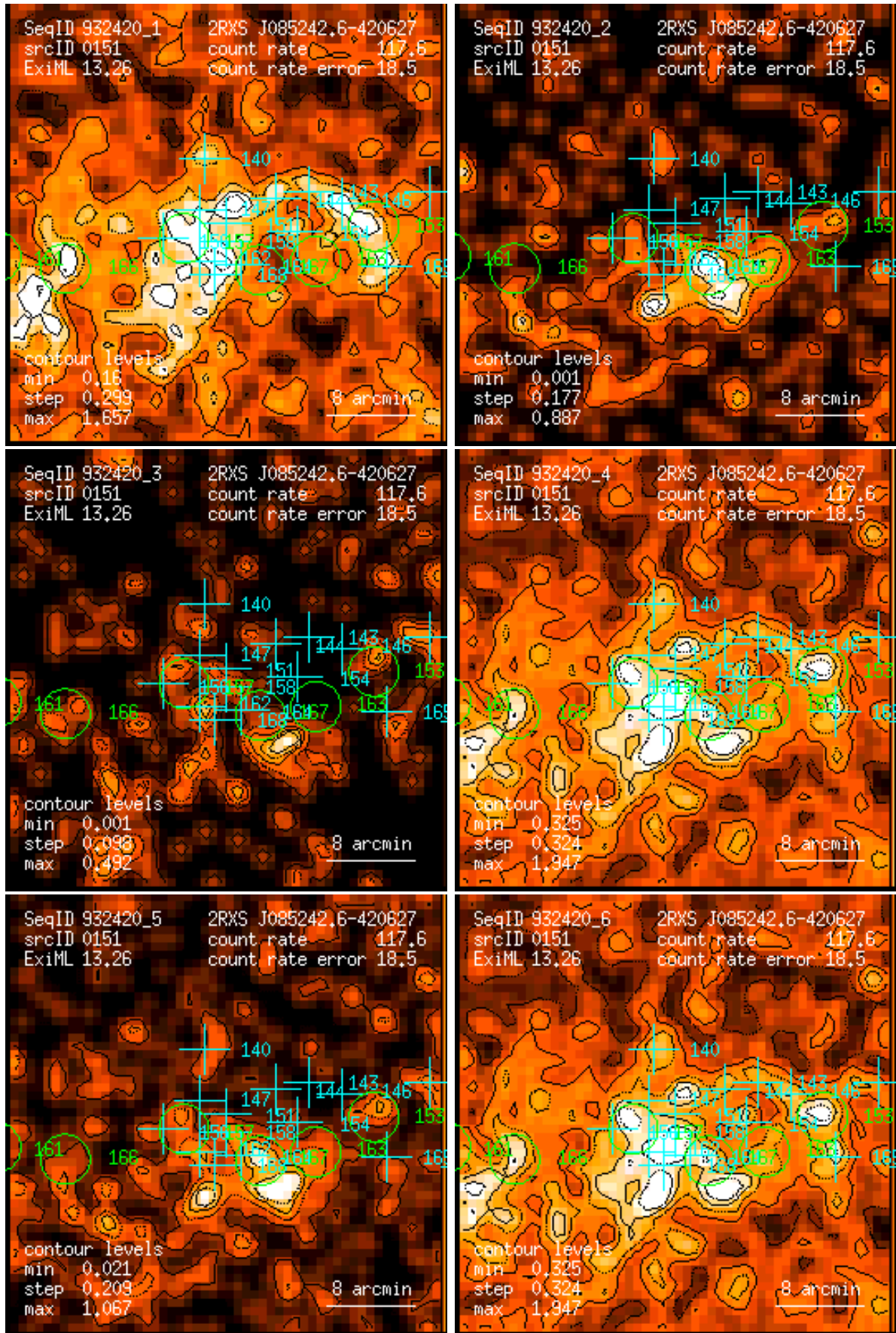
Figure 151: RASS 932420: detection 0151: band rate images, Gaussian filter: (1) PSPC channels 11 – 41, (2) 52 – 90, (3) 91 – 201, (4) 11 – 235, (5) 52 – 201, (6) 11 – 201. Broad band rates in counts/ks. Band rate contour levels in counts/ks/arcmin 2 .
