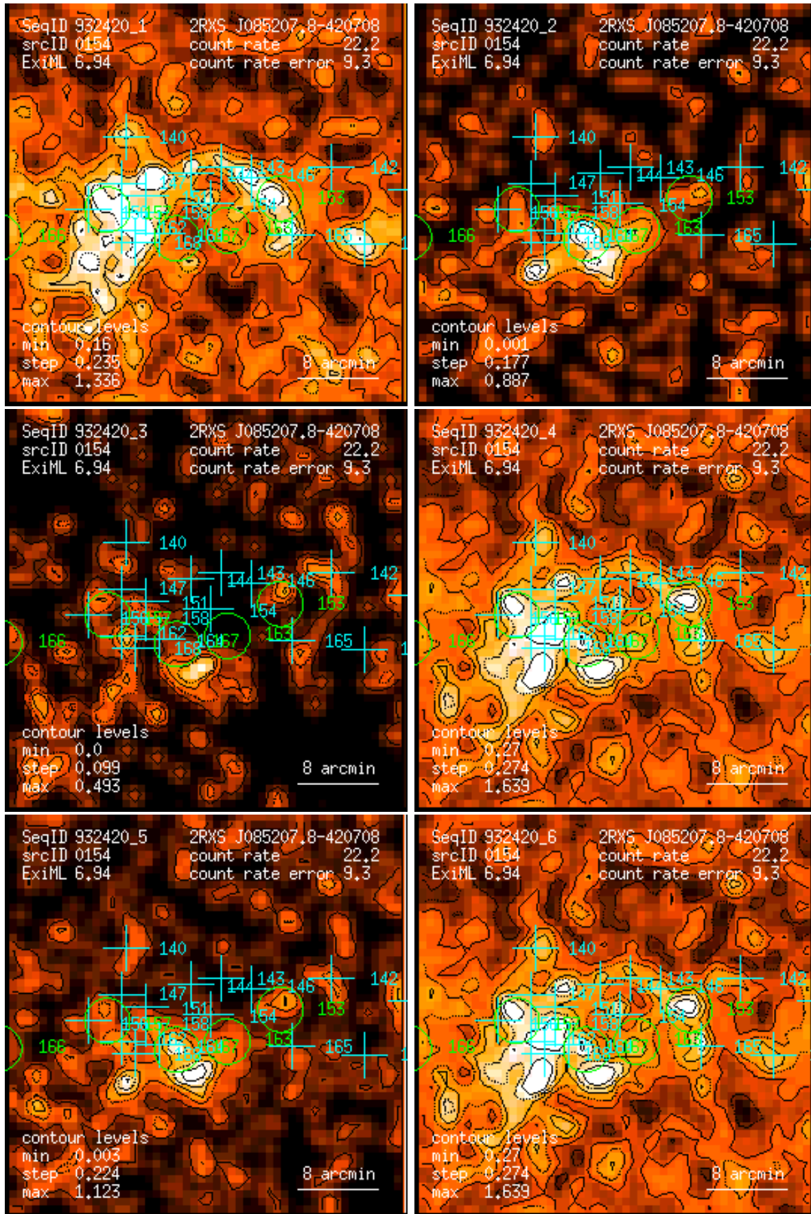
Figure 154: RASS 932420: detection 0154: band rate images, Gaussian filter: (1) PSPC channels 11 – 41, (2) 52 – 90, (3) 91 – 201, (4) 11 – 235, (5) 52 – 201, (6) 11 – 201. Broad band rates in counts/ks. Band rate contour levels in counts/ks/arcmin 2 .
