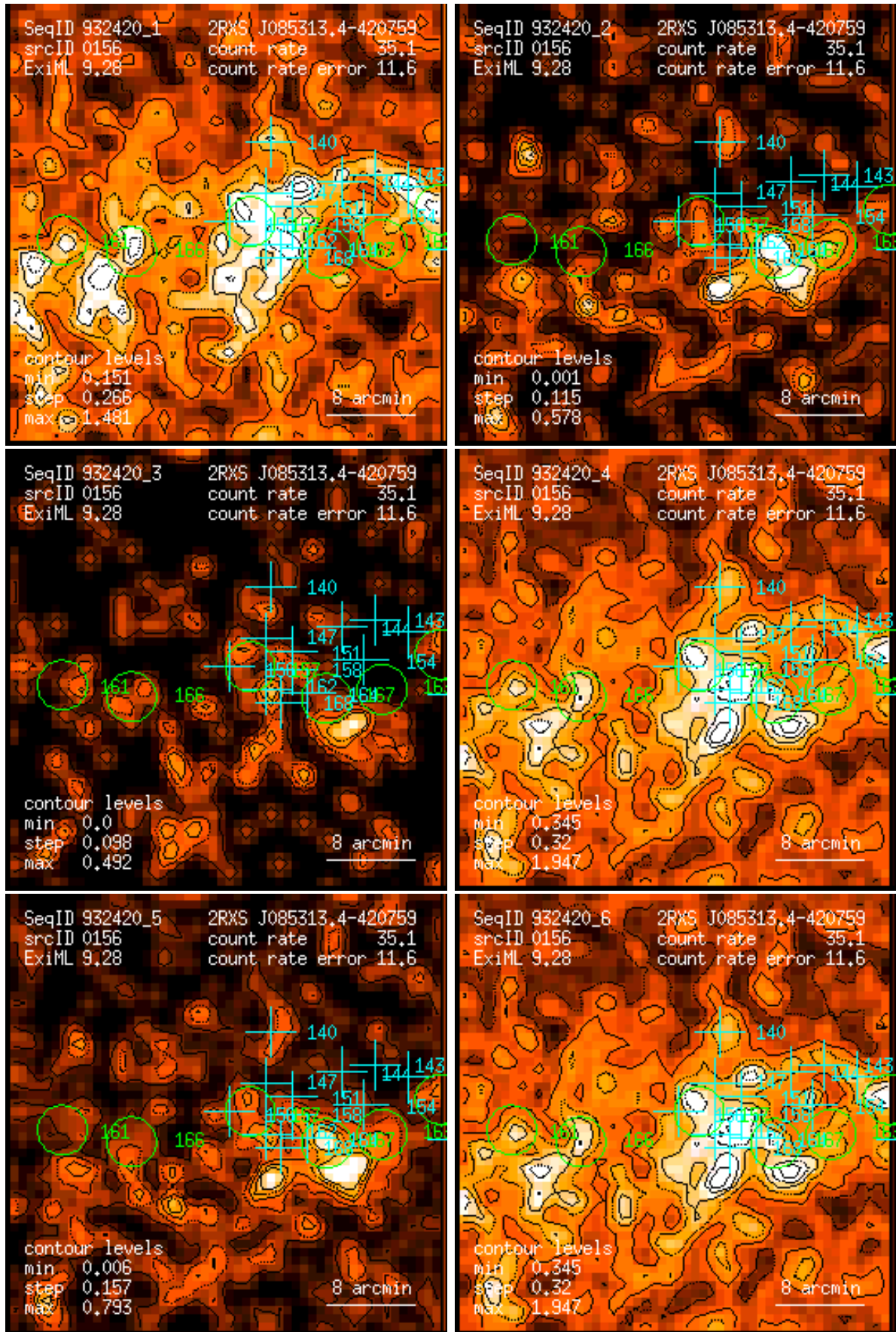
Figure 156: RASS 932420: detection 0156: band rate images, Gaussian filter: (1) PSPC channels 11 – 41, (2) 52 – 90, (3) 91 – 201, (4) 11 – 235, (5) 52 – 201, (6) 11 – 201. Broad band rates in counts/ks. Band rate contour levels in counts/ks/arcmin 2 .
