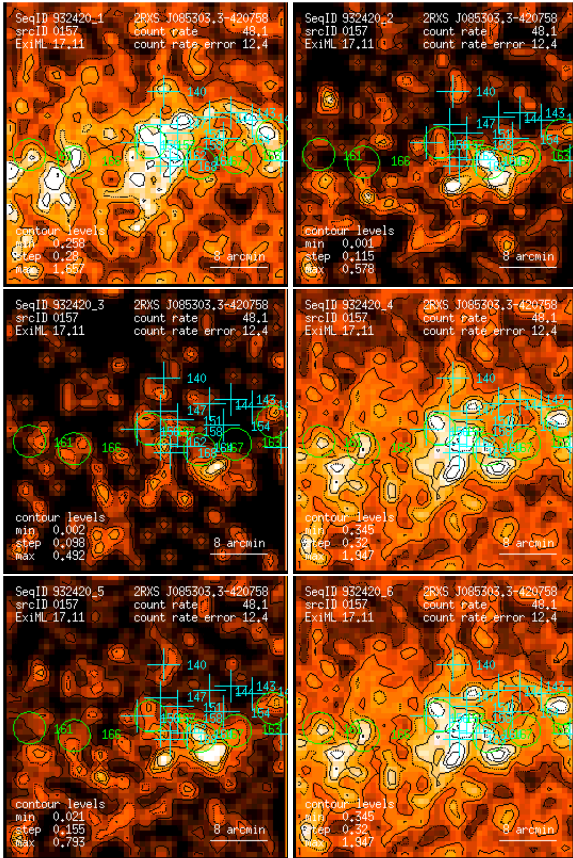
Figure 157: RASS 932420: detection 0157: band rate images, Gaussian filter: (1) PSPC channels 11 – 41, (2) 52 – 90, (3) 91 – 201, (4) 11 – 235, (5) 52 – 201, (6) 11 – 201. Broad band rates in counts/ks. Band rate contour levels in counts/ks/arcmin 2 .
