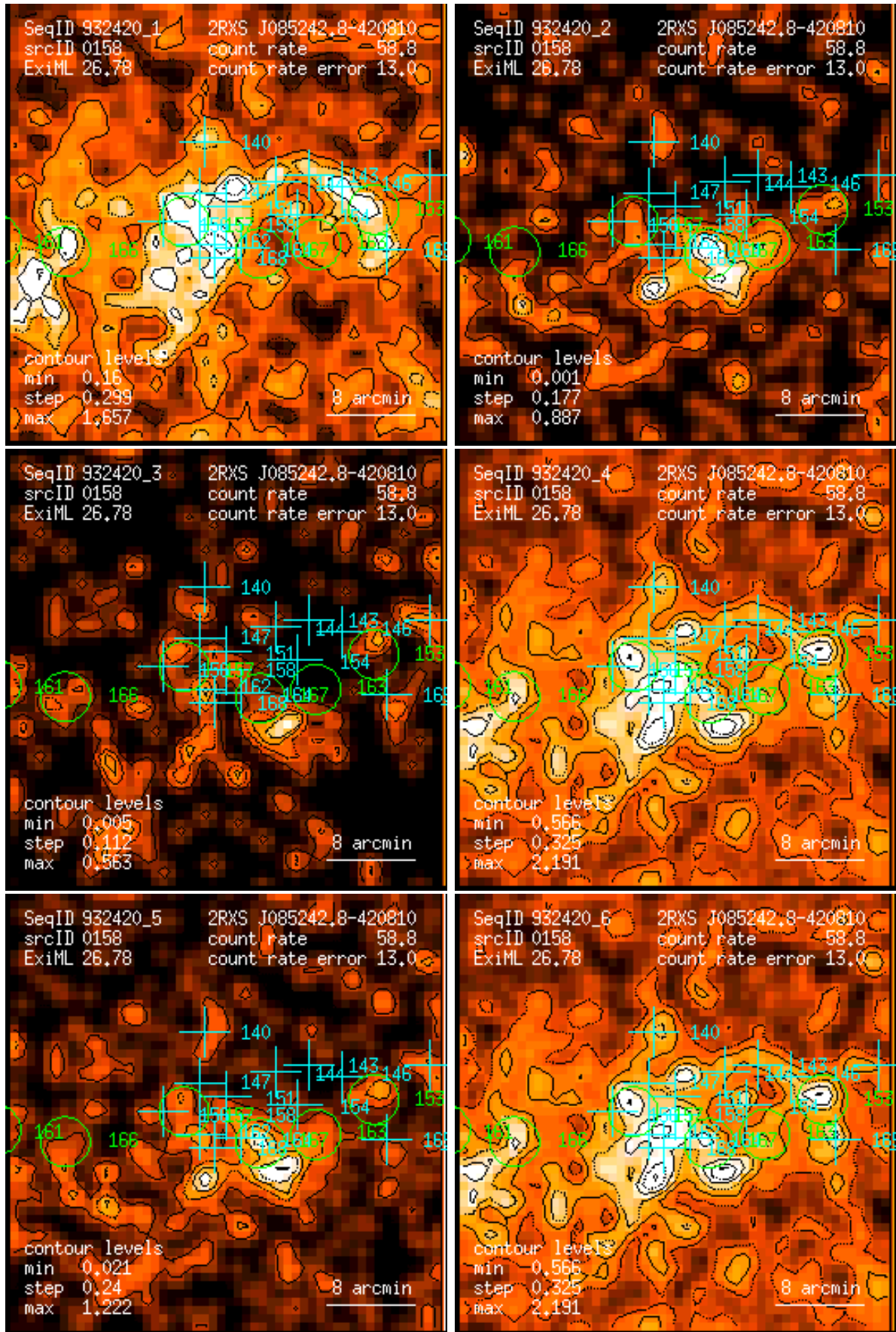
Figure 158: RASS 932420: detection 0158: band rate images, Gaussian filter: (1) PSPC channels 11 – 41, (2) 52 – 90, (3) 91 – 201, (4) 11 – 235, (5) 52 – 201, (6) 11 – 201. Broad band rates in counts/ks. Band rate contour levels in counts/ks/arcmin 2 .
