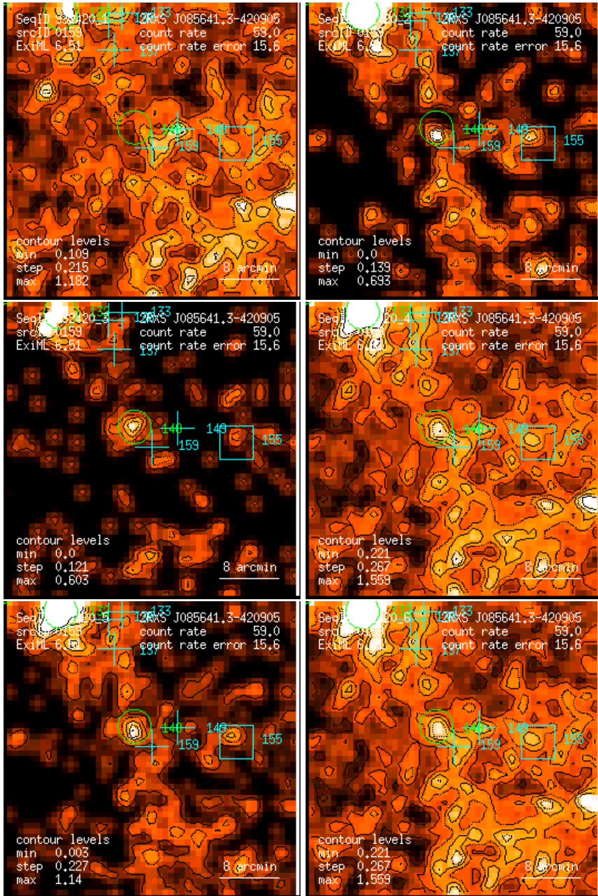
Figure 159: RASS 932420: detection 0159: band rate images, Gaussian filter: (1) PSPC channels 11 – 41, (2) 52 – 90, (3) 91 – 201, (4) 11 – 235, (5) 52 – 201, (6) 11 – 201. Broad band rates in counts/ks. Band rate contour levels in counts/ks/arcmin 2 .
