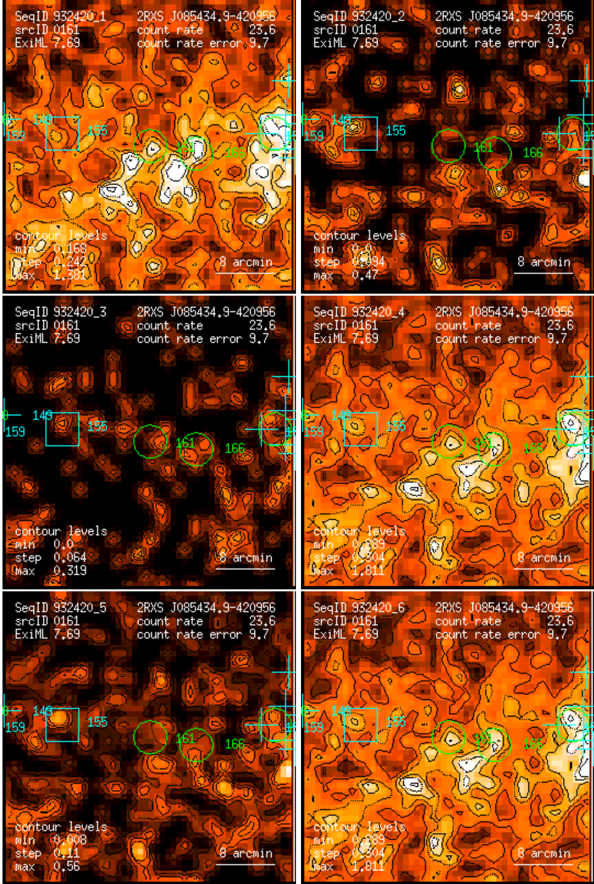
Figure 161: RASS 932420: detection 0161: band rate images, Gaussian filter: (1) PSPC channels 11 – 41, (2) 52 – 90, (3) 91 – 201, (4) 11 – 235, (5) 52 – 201, (6) 11 – 201. Broad band rates in counts/ks. Band rate contour levels in counts/ks/arcmin 2 .
