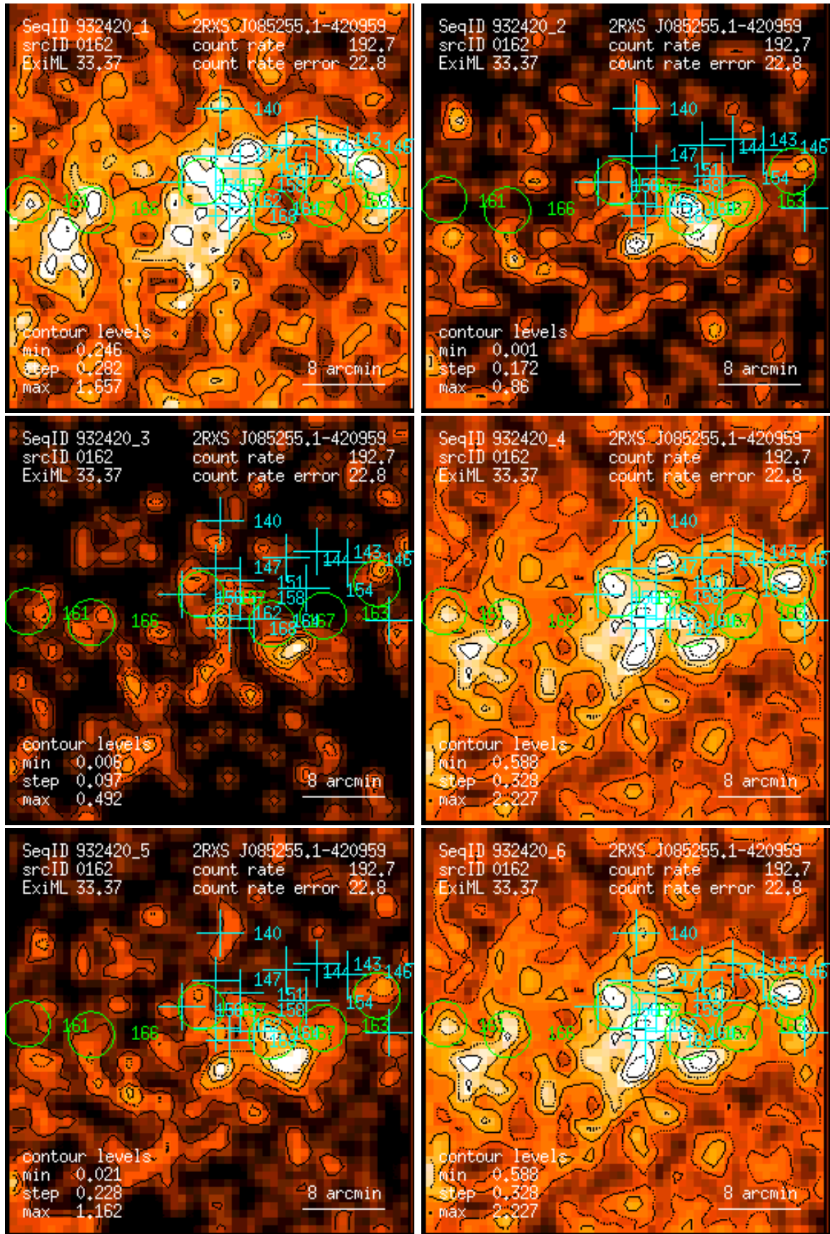
Figure 162: RASS 932420: detection 0162: band rate images, Gaussian filter: (1) PSPC channels 11 – 41, (2) 52 – 90, (3) 91 – 201, (4) 11 – 235, (5) 52 – 201, (6) 11 – 201. Broad band rates in counts/ks. Band rate contour levels in counts/ks/arcmin 2 .
