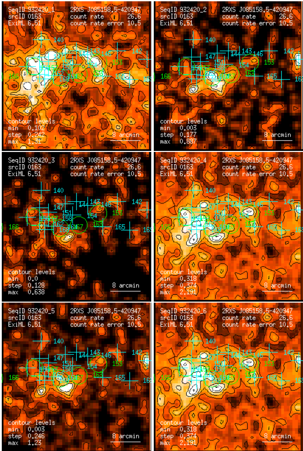
Figure 163: RASS 932420: detection 0163: band rate images, Gaussian filter: (1) PSPC channels 11 – 41, (2) 52 – 90, (3) 91 – 201, (4) 11 – 235, (5) 52 – 201, (6) 11 – 201. Broad band rates in counts/ks. Band rate contour levels in counts/ks/arcmin 2 .
