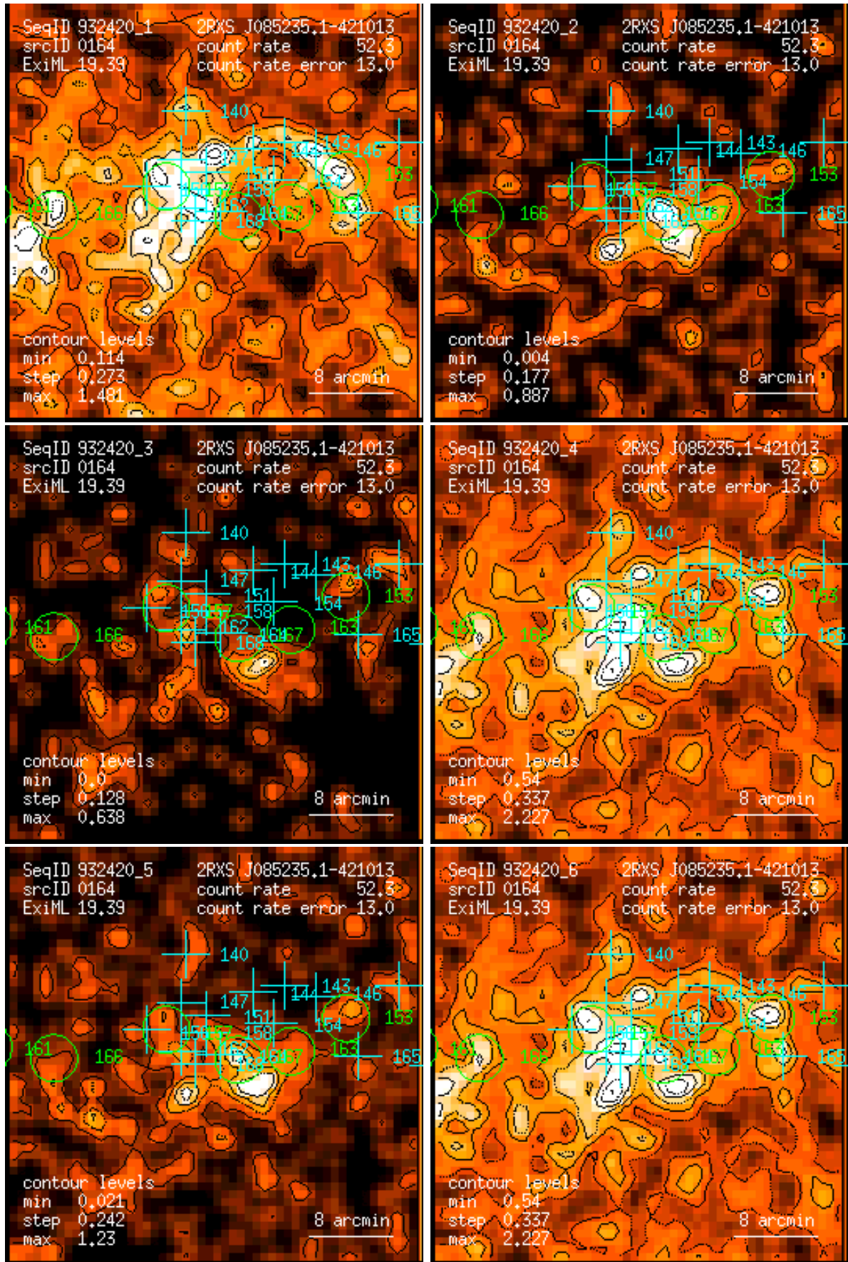
Figure 164: RASS 932420: detection 0164: band rate images, Gaussian filter: (1) PSPC channels 11 – 41, (2) 52 – 90, (3) 91 – 201, (4) 11 – 235, (5) 52 – 201, (6) 11 – 201. Broad band rates in counts/ks. Band rate contour levels in counts/ks/arcmin 2 .
