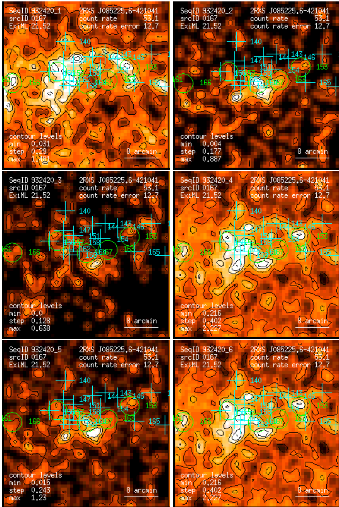
Figure 167: RASS 932420: detection 0167: band rate images, Gaussian filter: (1) PSPC channels 11 – 41, (2) 52 – 90, (3) 91 – 201, (4) 11 – 235, (5) 52 – 201, (6) 11 – 201. Broad band rates in counts/ks. Band rate contour levels in counts/ks/arcmin 2 .
