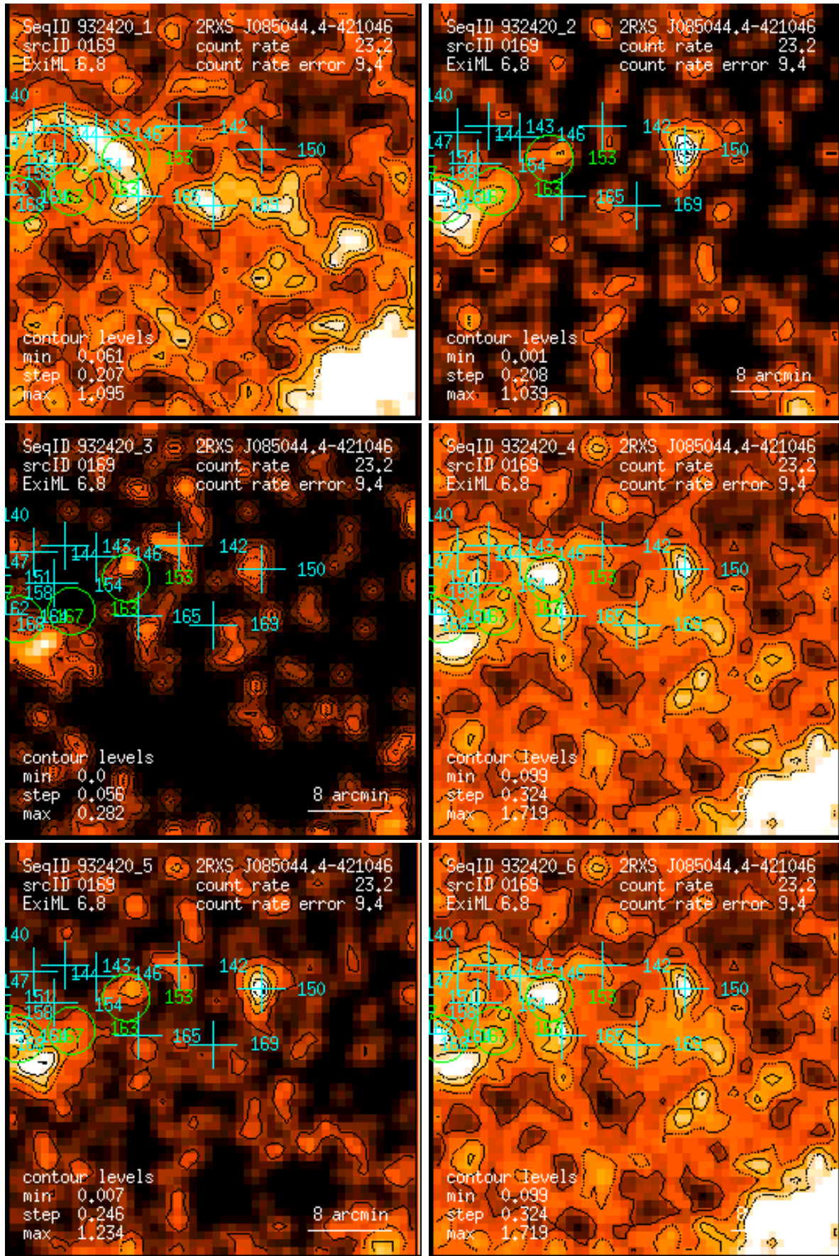
Figure 169: RASS 932420: detection 0169: band rate images, Gaussian filter: (1) PSPC channels 11 – 41, (2) 52 – 90, (3) 91 – 201, (4) 11 – 235, (5) 52 – 201, (6) 11 – 201. Broad band rates in counts/ks. Band rate contour levels in counts/ks/arcmin 2 .
