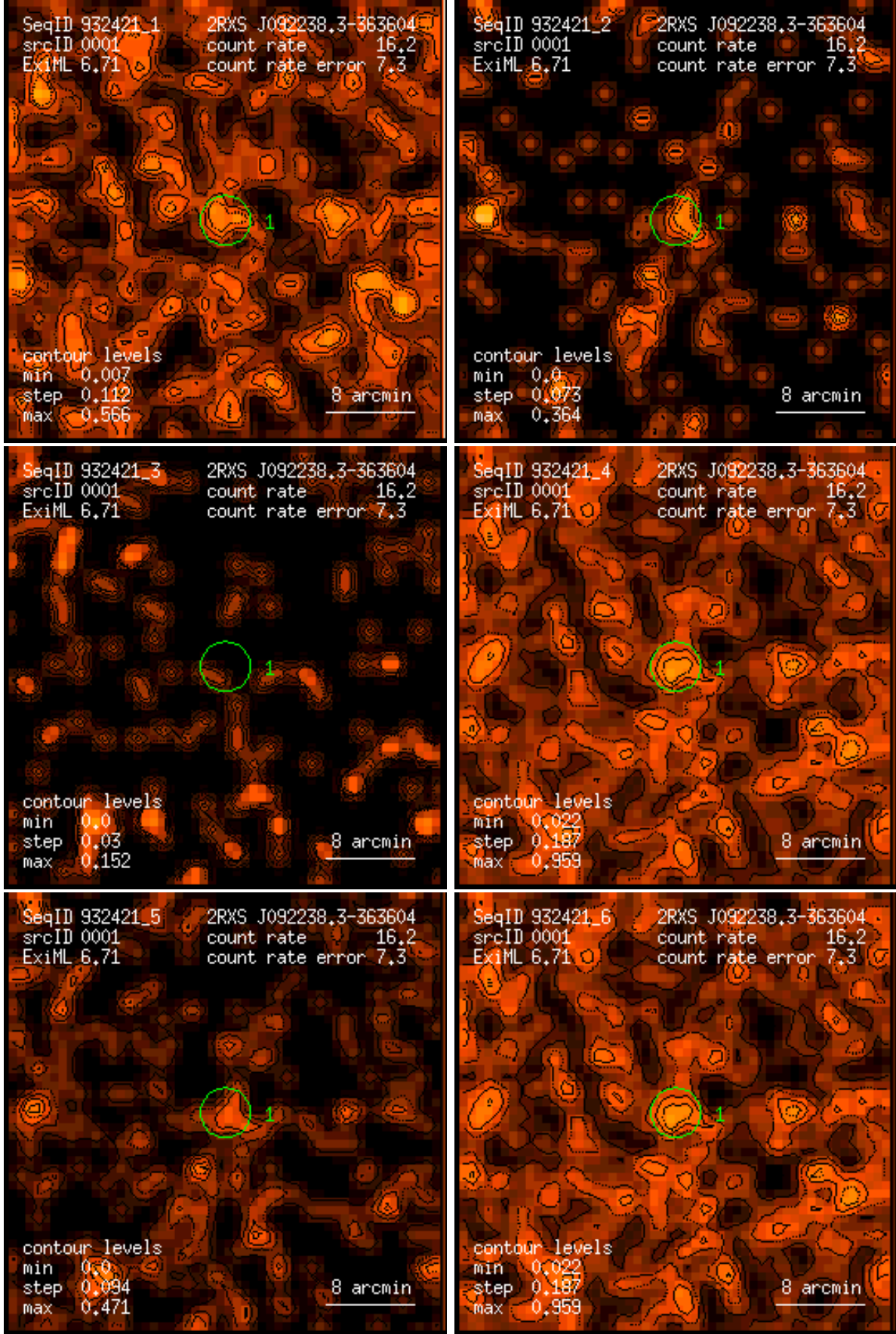
Figure 1: RASS 932421: detection 0001: band rate images, Gaussian filter: (1) PSPC channels 11 – 41, (2) 52 – 90, (3) 91 – 201, (4) 11 – 235, (5) 52 – 201, (6) 11 – 201. Broad band rates in counts/ks. Band rate contour levels in counts/ks/arcmin 2 .
