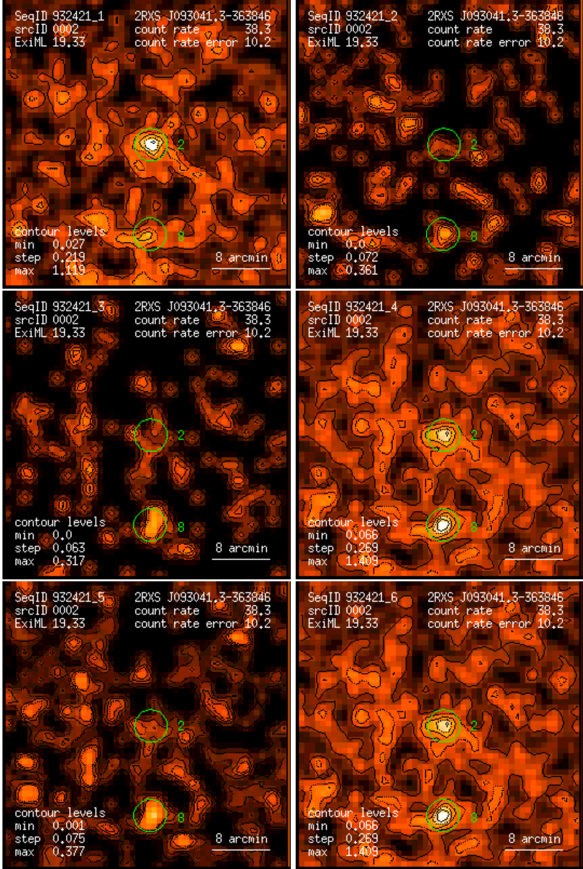
Figure 2: RASS 932421: detection 0002: band rate images, Gaussian filter: (1) PSPC channels 11 – 41, (2) 52 – 90, (3) 91 – 201, (4) 11 – 235, (5) 52 – 201, (6) 11 – 201. Broad band rates in counts/ks. Band rate contour levels in counts/ks/arcmin 2 .
