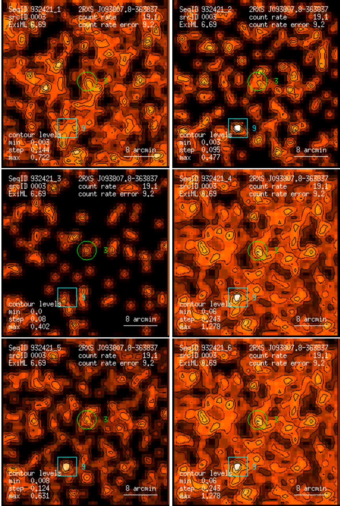
Figure 3: RASS 932421: detection 0003: band rate images, Gaussian filter: (1) PSPC channels 11 – 41, (2) 52 – 90, (3) 91 – 201, (4) 11 – 235, (5) 52 – 201, (6) 11 – 201. Broad band rates in counts/ks. Band rate contour levels in counts/ks/arcmin 2 .
