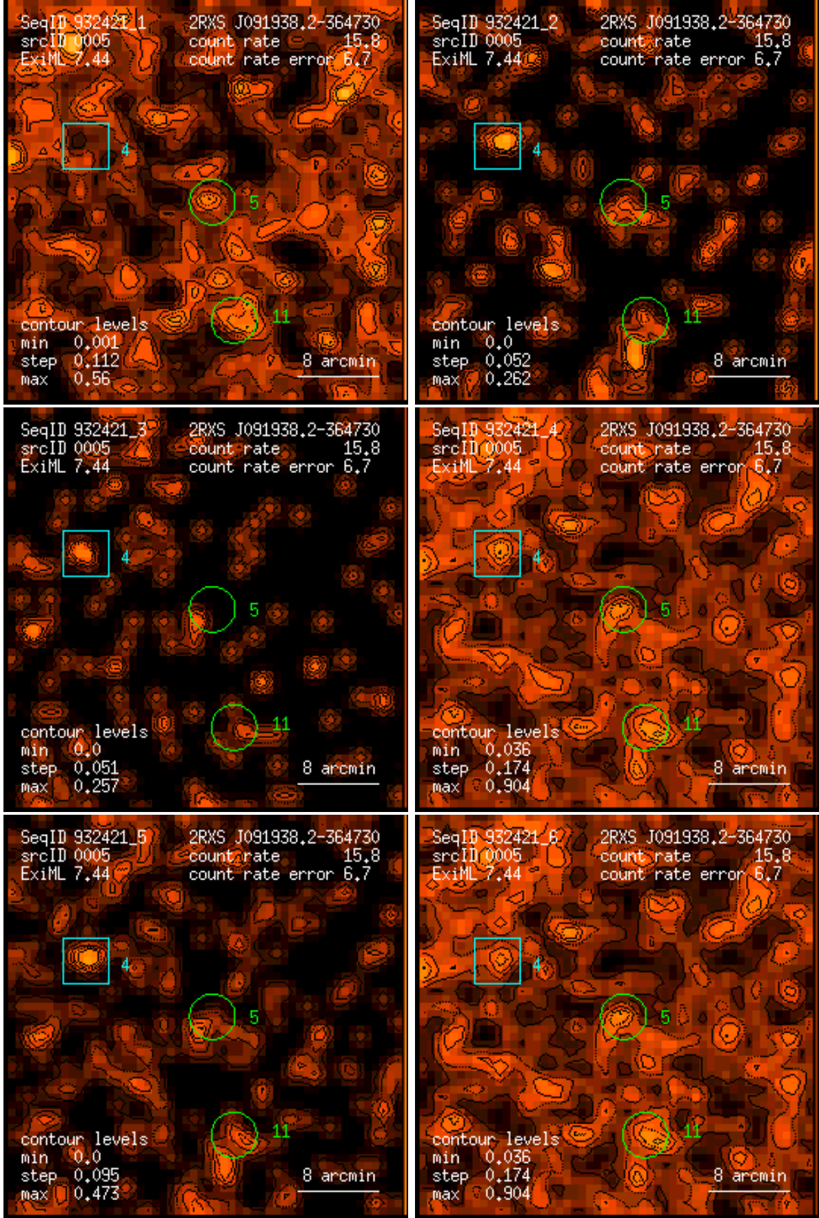
Figure 5: RASS 932421: detection 0005: band rate images, Gaussian filter: (1) PSPC channels 11 – 41, (2) 52 – 90, (3) 91 – 201, (4) 11 – 235, (5) 52 – 201, (6) 11 – 201. Broad band rates in counts/ks. Band rate contour levels in counts/ks/arcmin 2 .
