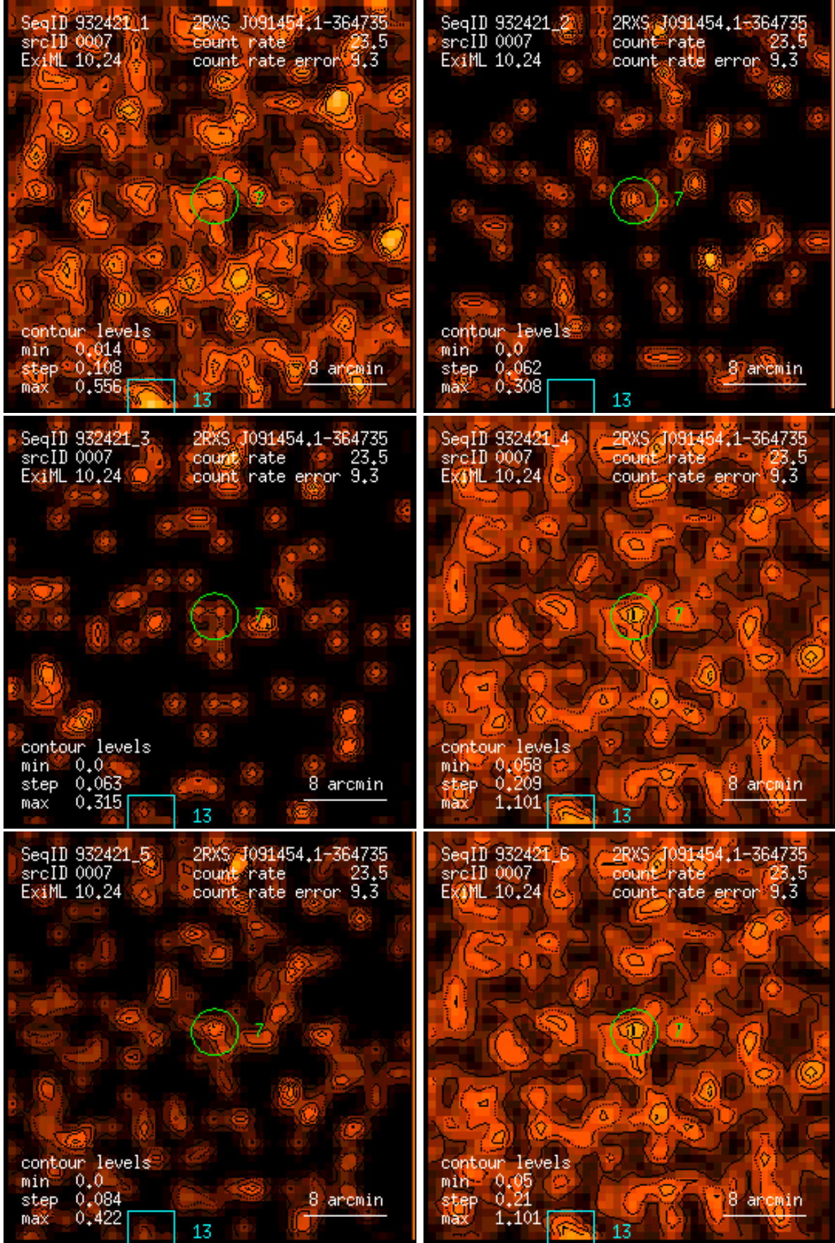
Figure 7: RASS 932421: detection 0007: band rate images, Gaussian filter: (1) PSPC channels 11 – 41, (2) 52 – 90, (3) 91 – 201, (4) 11 – 235, (5) 52 – 201, (6) 11 – 201. Broad band rates in counts/ks. Band rate contour levels in counts/ks/arcmin 2 .
