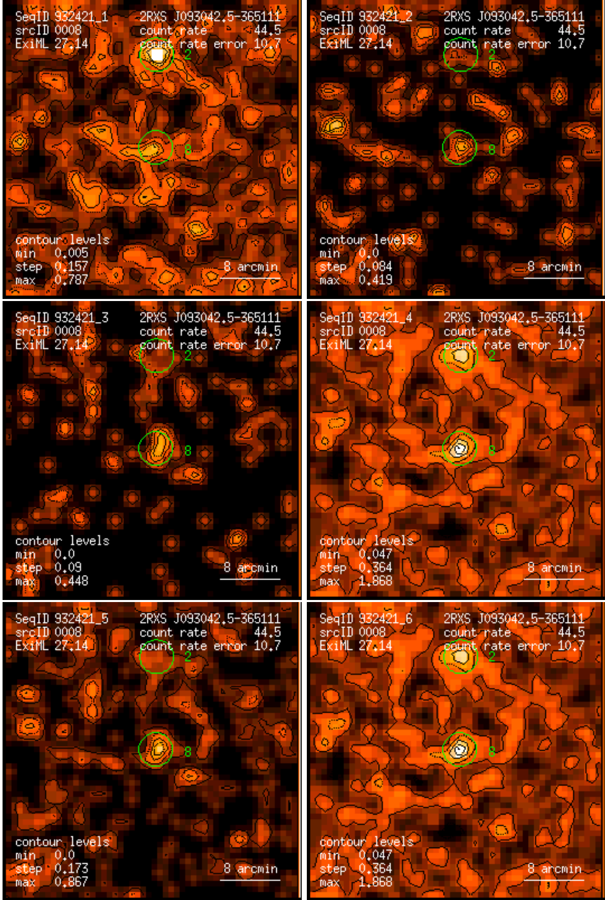
Figure 8: RASS 932421: detection 0008: band rate images, Gaussian filter: (1) PSPC channels 11 – 41, (2) 52 – 90, (3) 91 – 201, (4) 11 – 235, (5) 52 – 201, (6) 11 – 201. Broad band rates in counts/ks. Band rate contour levels in counts/ks/arcmin 2 .
