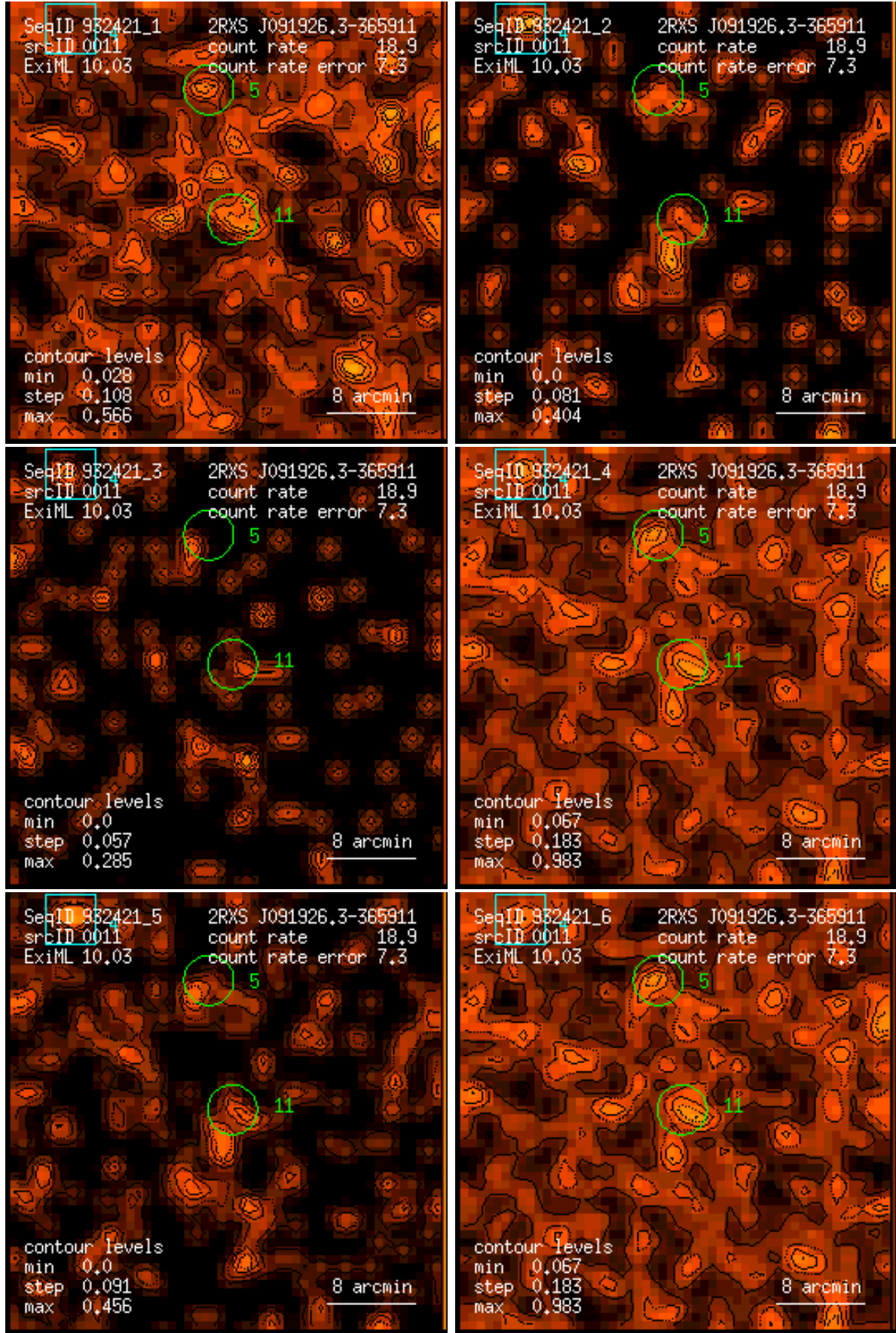
Figure 11: RASS 932421: detection 0011: band rate images, Gaussian filter: (1) PSPC channels 11 – 41, (2) 52 – 90, (3) 91 – 201, (4) 11 – 235, (5) 52 – 201, (6) 11 – 201. Broad band rates in counts/ks. Band rate contour levels in counts/ks/arcmin 2 .
