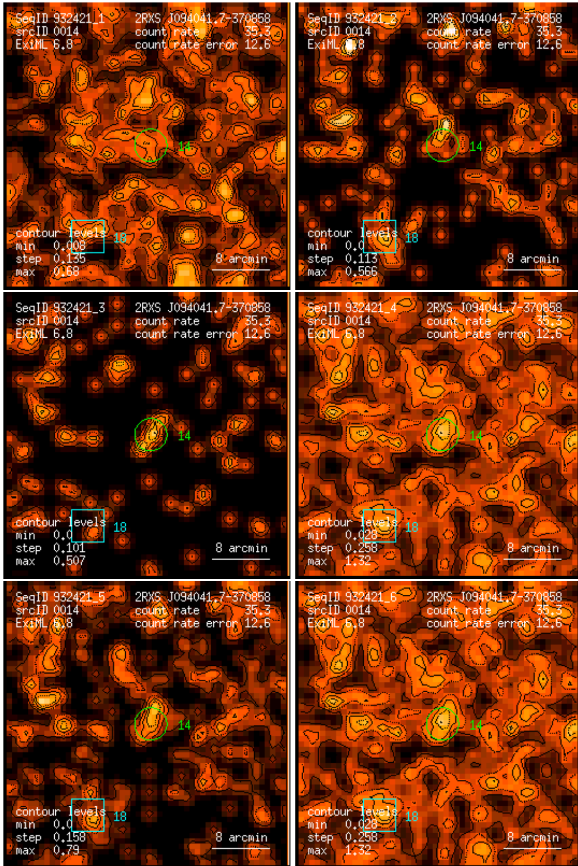
Figure 14: RASS 932421: detection 0014: band rate images, Gaussian filter: (1) PSPC channels 11 – 41, (2) 52 – 90, (3) 91 – 201, (4) 11 – 235, (5) 52 – 201, (6) 11 – 201. Broad band rates in counts/ks. Band rate contour levels in counts/ks/arcmin 2 .
