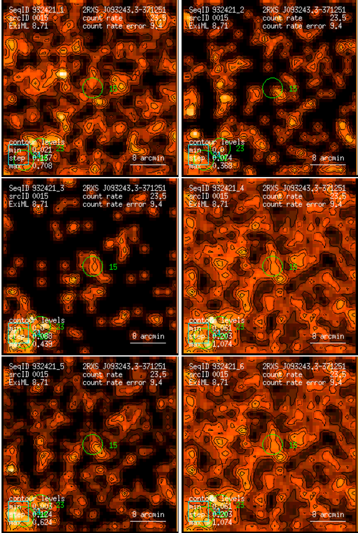
Figure 15: RASS 932421: detection 0015: band rate images, Gaussian filter: (1) PSPC channels 11 – 41, (2) 52 – 90, (3) 91 – 201, (4) 11 – 235, (5) 52 – 201, (6) 11 – 201. Broad band rates in counts/ks. Band rate contour levels in counts/ks/arcmin 2 .
