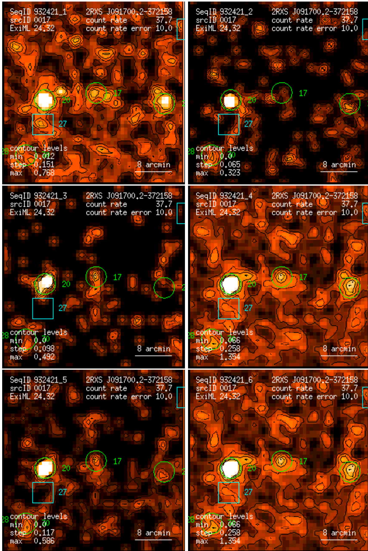
Figure 17: RASS 932421: detection 0017: band rate images, Gaussian filter: (1) PSPC channels 11 – 41, (2) 52 – 90, (3) 91 – 201, (4) 11 – 235, (5) 52 – 201, (6) 11 – 201. Broad band rates in counts/ks. Band rate contour levels in counts/ks/arcmin 2 .
