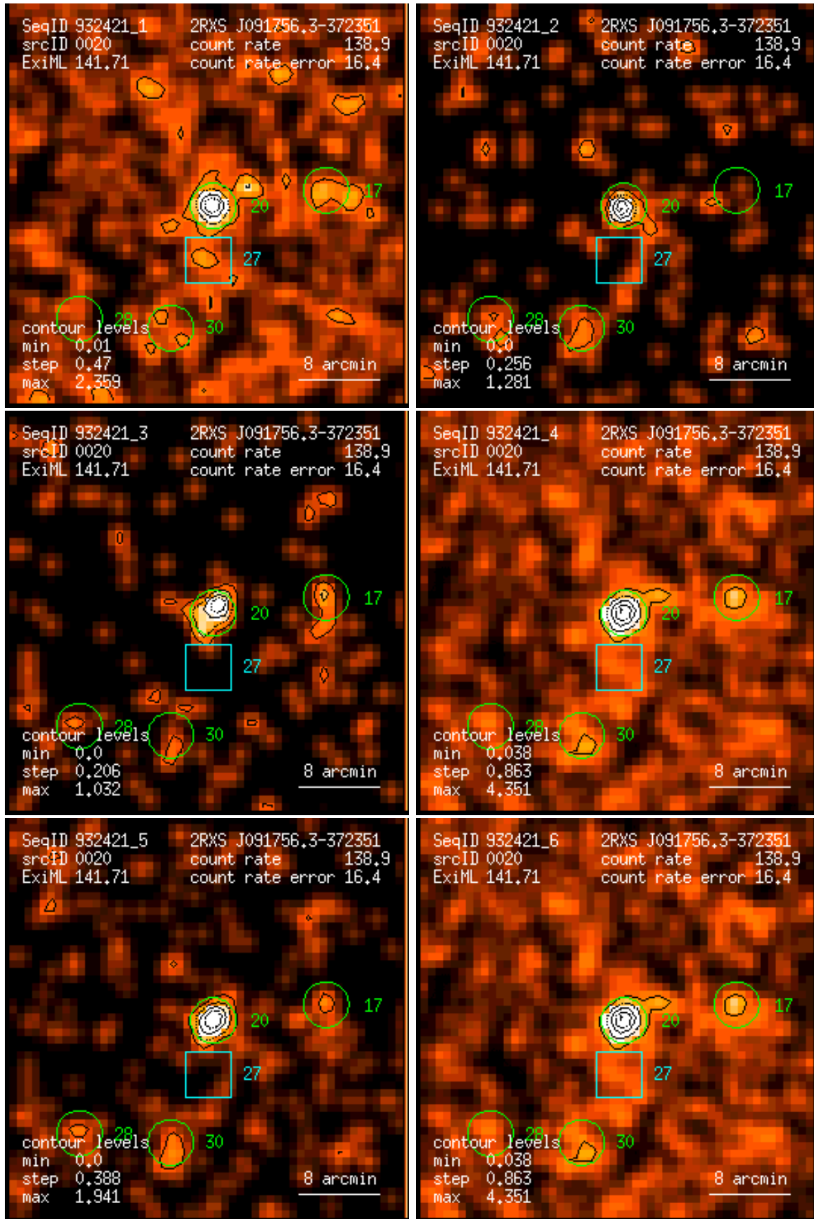
Figure 20: RASS 932421: detection 0020: band rate images, Gaussian filter: (1) PSPC channels 11 – 41, (2) 52 – 90, (3) 91 – 201, (4) 11 – 235, (5) 52 – 201, (6) 11 – 201. Broad band rates in counts/ks. Band rate contour levels in counts/ks/arcmin 2 .
