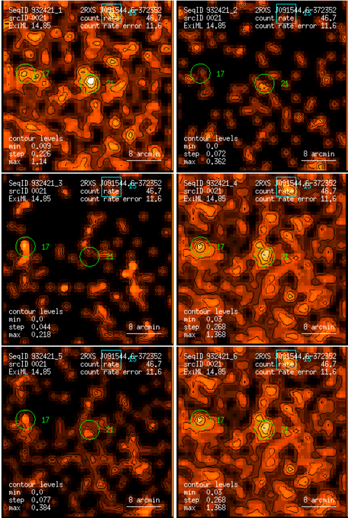
Figure 21: RASS 932421: detection 0021: band rate images, Gaussian filter: (1) PSPC channels 11 – 41, (2) 52 – 90, (3) 91 – 201, (4) 11 – 235, (5) 52 – 201, (6) 11 – 201. Broad band rates in counts/ks. Band rate contour levels in counts/ks/arcmin 2 .
