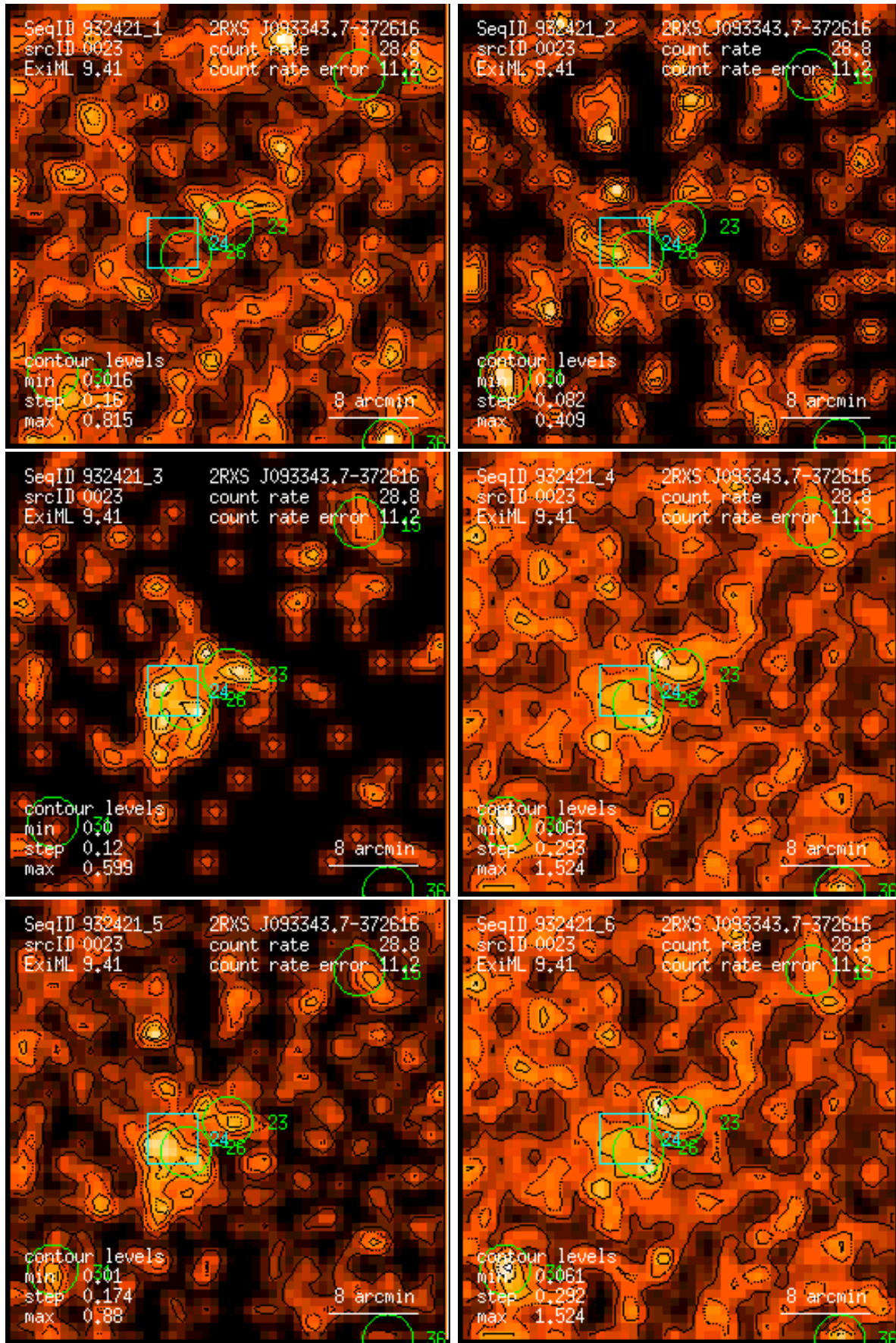
Figure 23: RASS 932421: detection 0023: band rate images, Gaussian filter: (1) PSPC channels 11 – 41, (2) 52 – 90, (3) 91 – 201, (4) 11 – 235, (5) 52 – 201, (6) 11 – 201. Broad band rates in counts/ks. Band rate contour levels in counts/ks/arcmin 2 .
