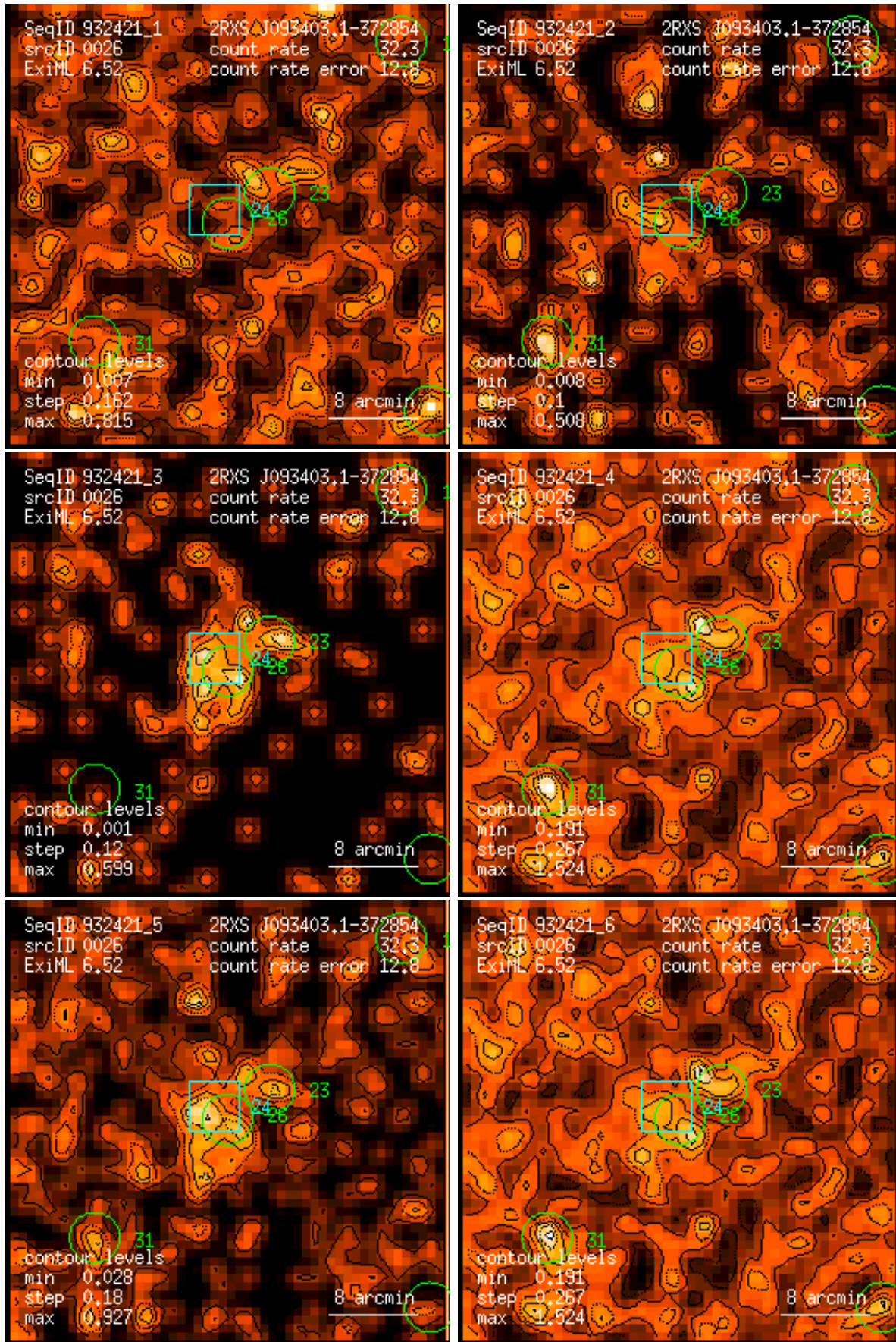
Figure 26: RASS 932421: detection 0026: band rate images, Gaussian filter: (1) PSPC channels 11 – 41, (2) 52 – 90, (3) 91 – 201, (4) 11 – 235, (5) 52 – 201, (6) 11 – 201. Broad band rates in counts/ks. Band rate contour levels in counts/ks/arcmin 2 .
