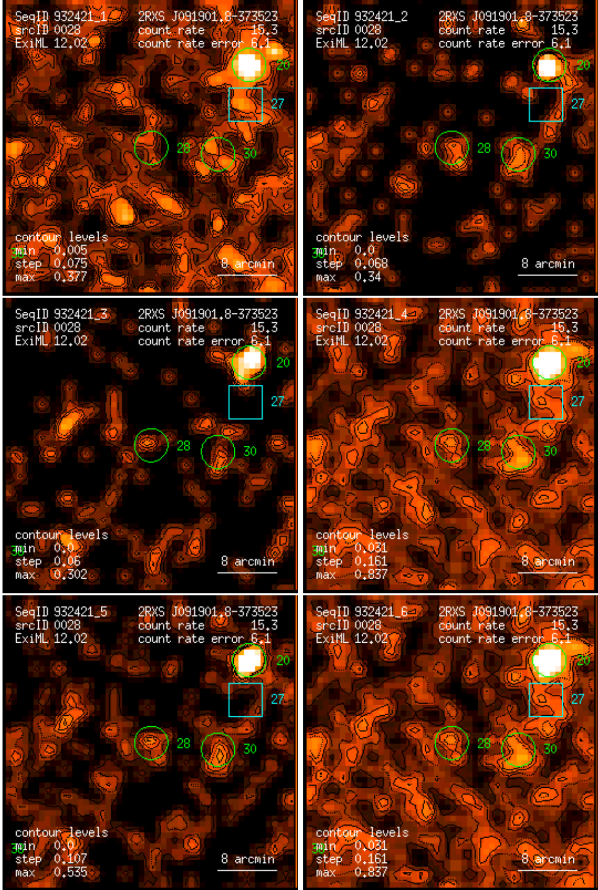
Figure 28: RASS 932421: detection 0028: band rate images, Gaussian filter: (1) PSPC channels 11 – 41, (2) 52 – 90, (3) 91 – 201, (4) 11 – 235, (5) 52 – 201, (6) 11 – 201. Broad band rates in counts/ks. Band rate contour levels in counts/ks/arcmin 2 .
