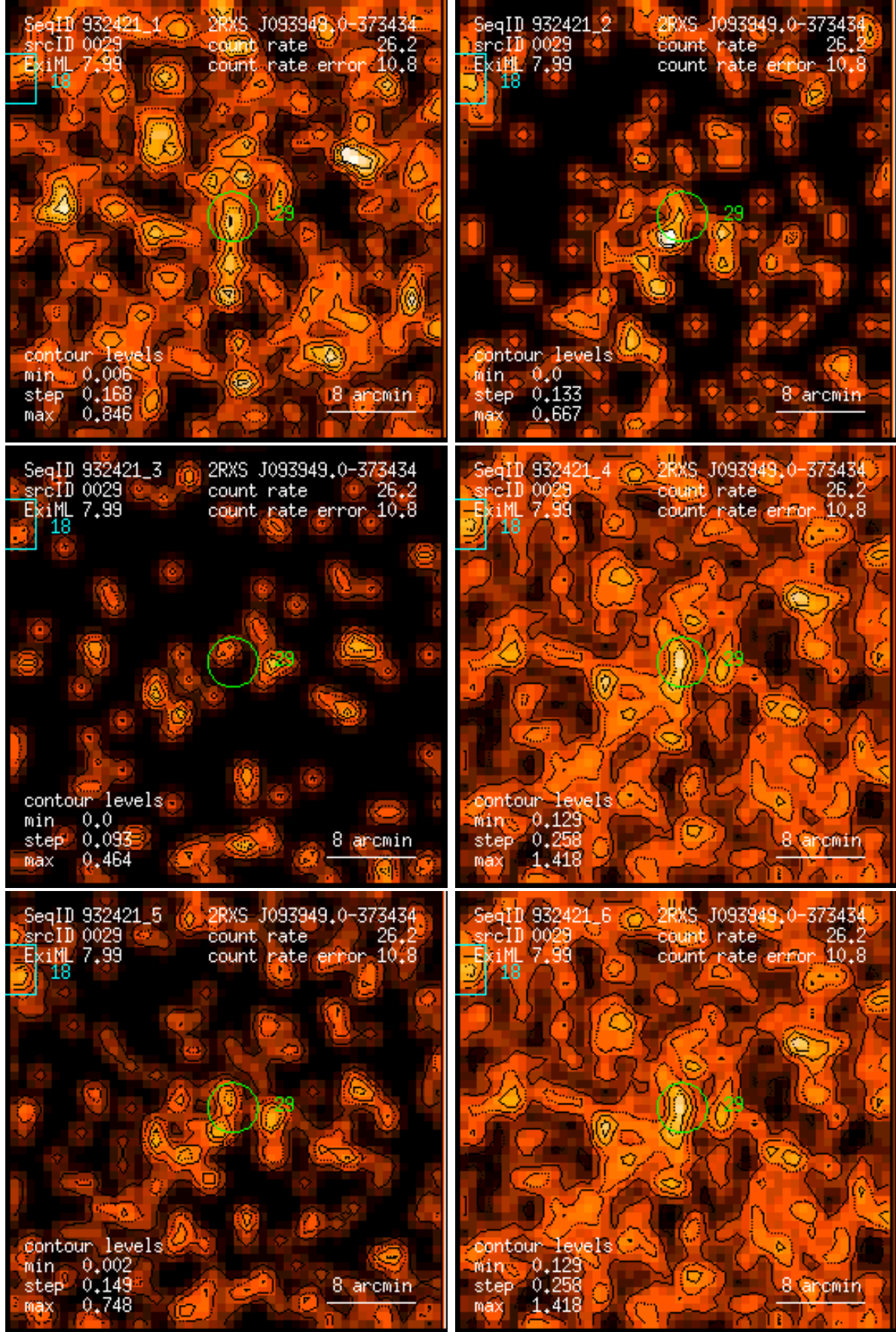
Figure 29: RASS 932421: detection 0029: band rate images, Gaussian filter: (1) PSPC channels 11 – 41, (2) 52 – 90, (3) 91 – 201, (4) 11 – 235, (5) 52 – 201, (6) 11 – 201. Broad band rates in counts/ks. Band rate contour levels in counts/ks/arcmin 2 .
