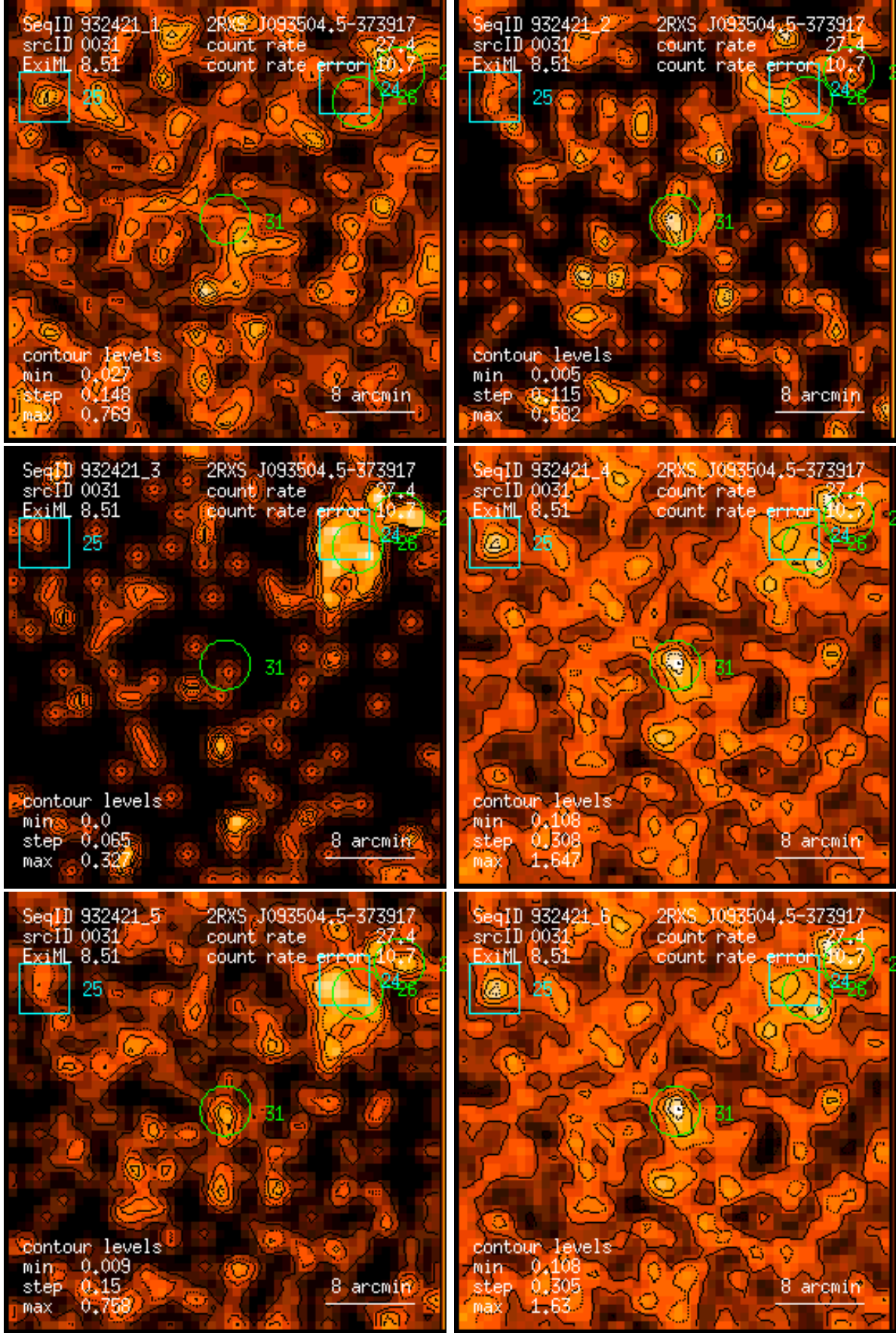
Figure 31: RASS 932421: detection 0031: band rate images, Gaussian filter: (1) PSPC channels 11 – 41, (2) 52 – 90, (3) 91 – 201, (4) 11 – 235, (5) 52 – 201, (6) 11 – 201. Broad band rates in counts/ks. Band rate contour levels in counts/ks/arcmin 2 .
