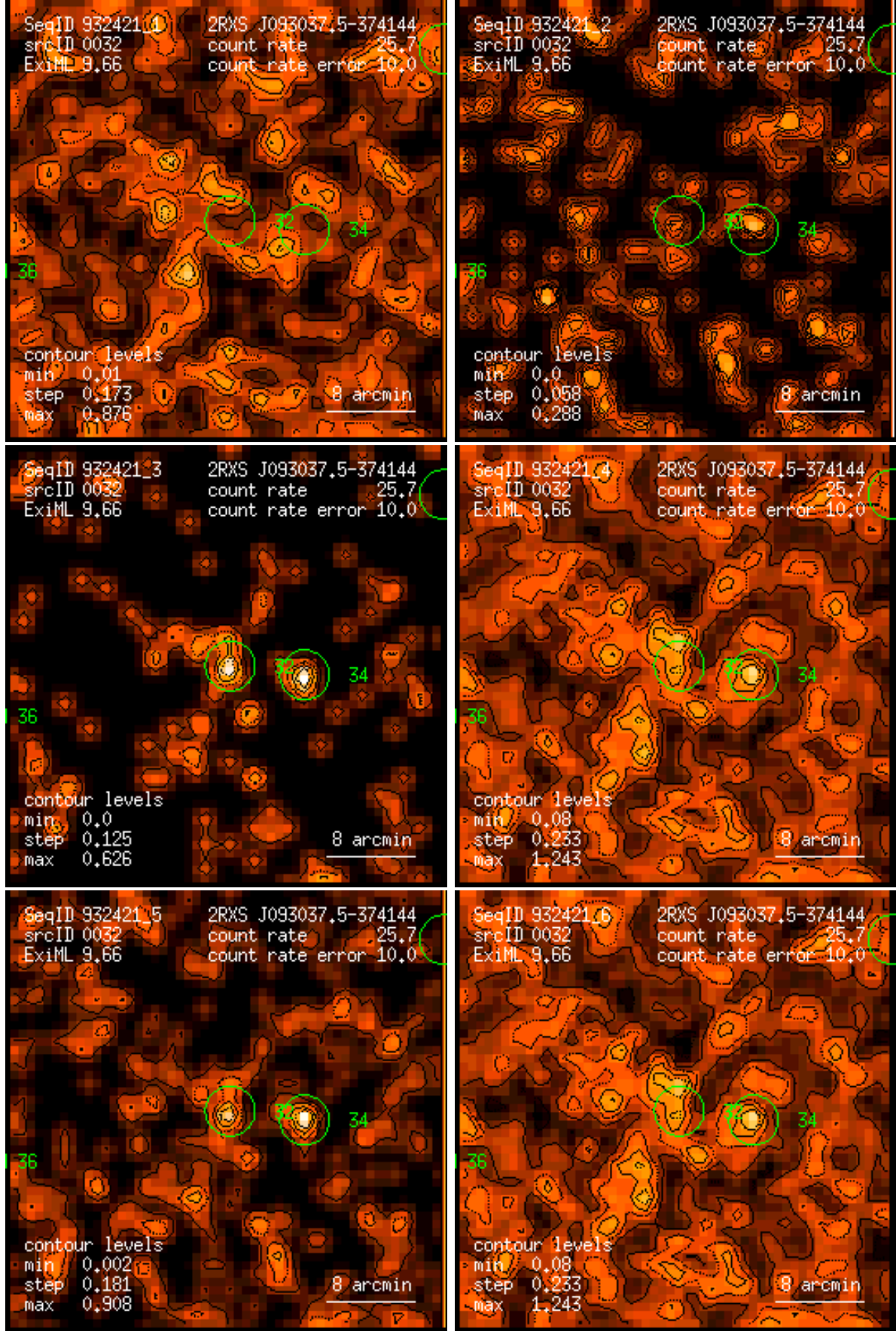
Figure 32: RASS 932421: detection 0032: band rate images, Gaussian filter: (1) PSPC channels 11 – 41, (2) 52 – 90, (3) 91 – 201, (4) 11 – 235, (5) 52 – 201, (6) 11 – 201. Broad band rates in counts/ks. Band rate contour levels in counts/ks/arcmin 2 .
