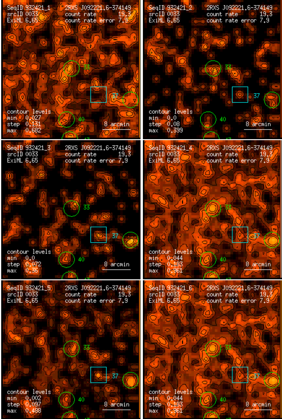
Figure 33: RASS 932421: detection 0033: band rate images, Gaussian filter: (1) PSPC channels 11 – 41, (2) 52 – 90, (3) 91 – 201, (4) 11 – 235, (5) 52 – 201, (6) 11 – 201. Broad band rates in counts/ks. Band rate contour levels in counts/ks/arcmin 2 .
