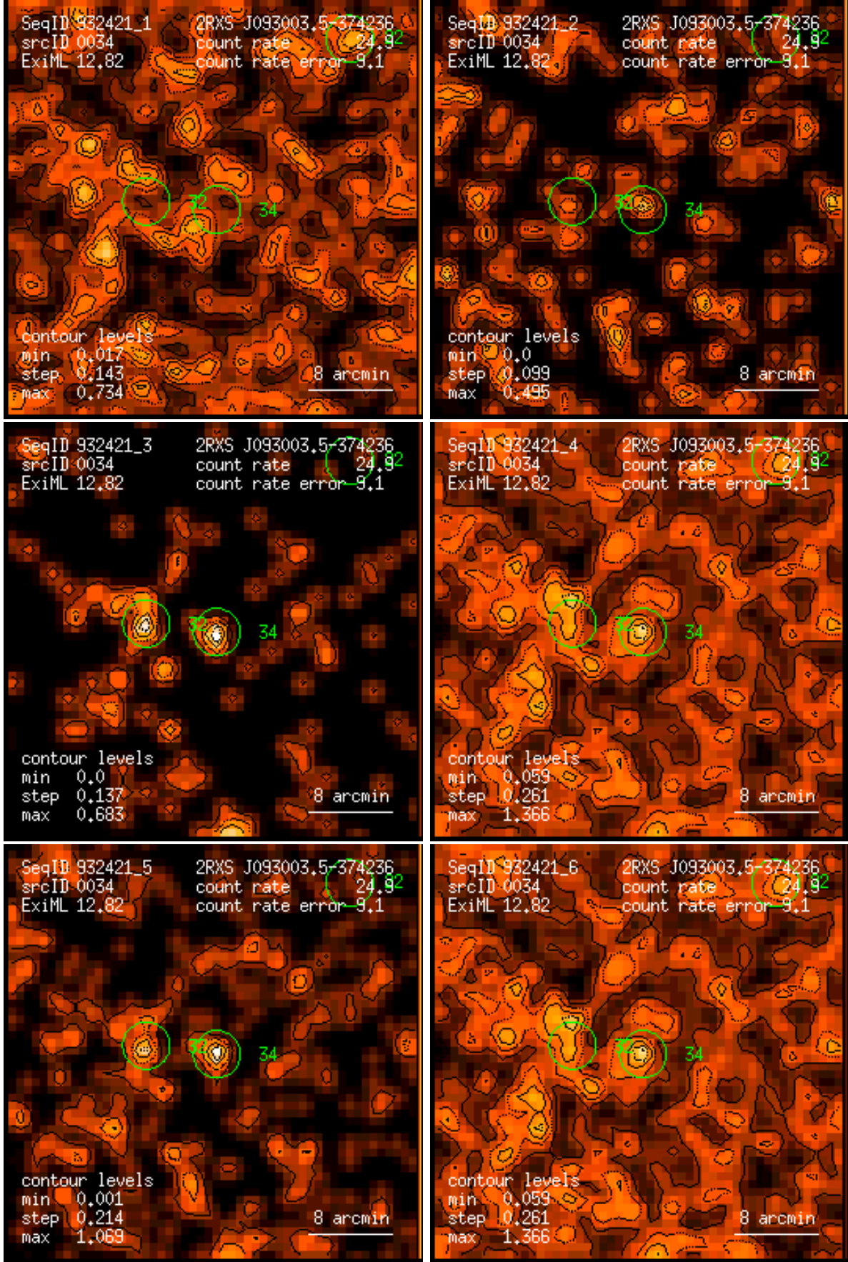
Figure 34: RASS 932421: detection 0034: band rate images, Gaussian filter: (1) PSPC channels 11 – 41, (2) 52 – 90, (3) 91 – 201, (4) 11 – 235, (5) 52 – 201, (6) 11 – 201. Broad band rates in counts/ks. Band rate contour levels in counts/ks/arcmin 2 .
