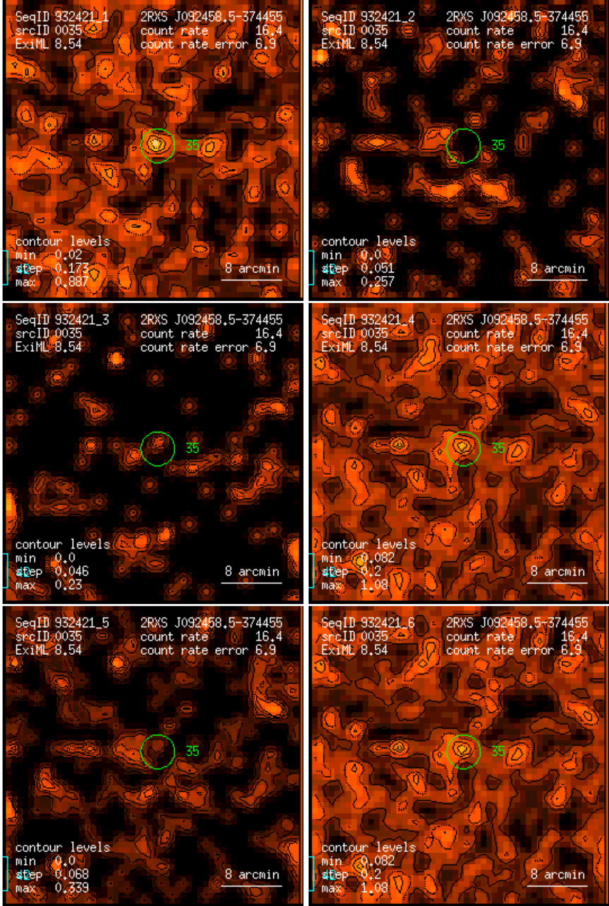
Figure 35: RASS 932421: detection 0035: band rate images, Gaussian filter: (1) PSPC channels 11 – 41, (2) 52 – 90, (3) 91 – 201, (4) 11 – 235, (5) 52 – 201, (6) 11 – 201. Broad band rates in counts/ks. Band rate contour levels in counts/ks/arcmin 2 .
