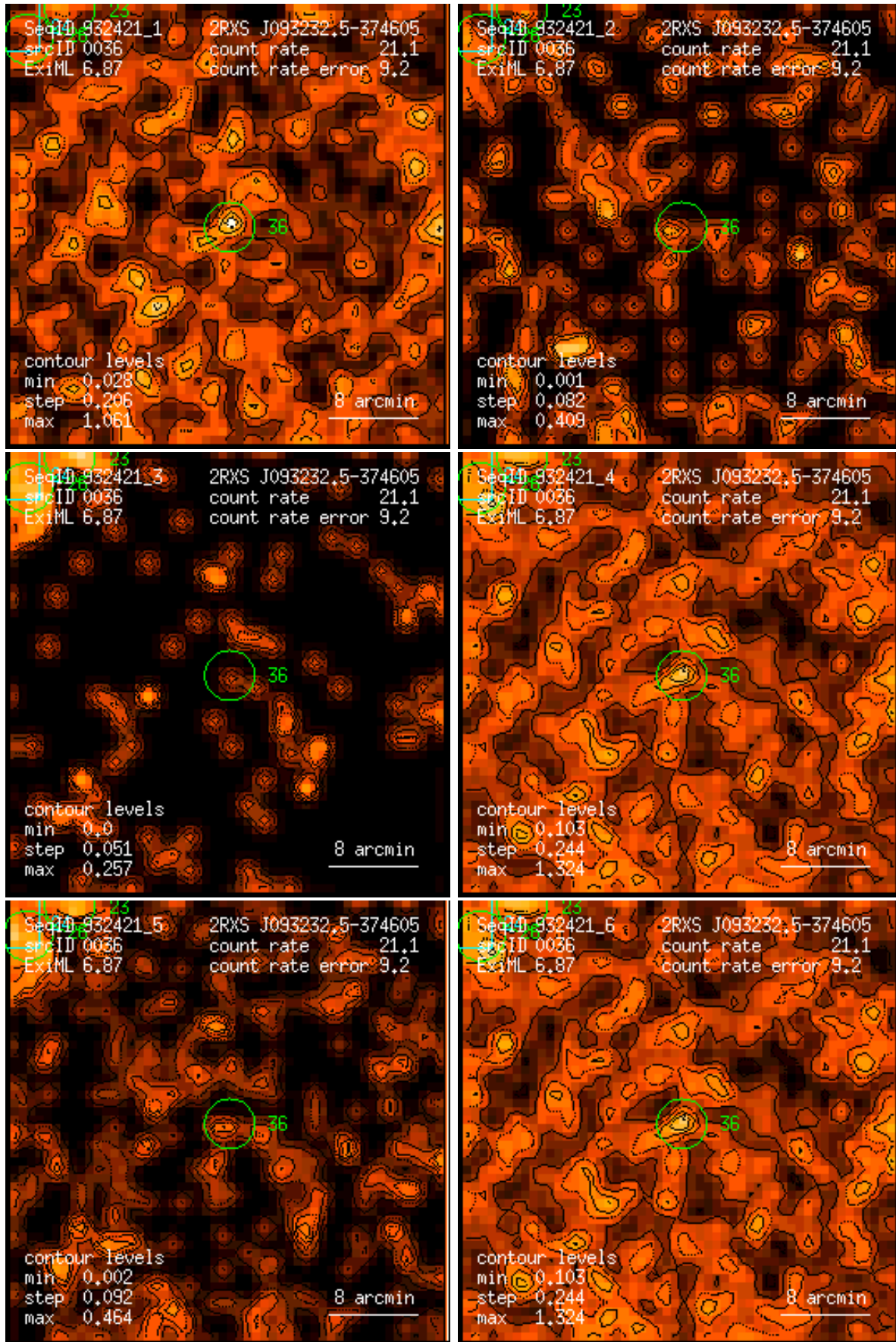
Figure 36: RASS 932421: detection 0036: band rate images, Gaussian filter: (1) PSPC channels 11 – 41, (2) 52 – 90, (3) 91 – 201, (4) 11 – 235, (5) 52 – 201, (6) 11 – 201. Broad band rates in counts/ks. Band rate contour levels in counts/ks/arcmin 2 .
