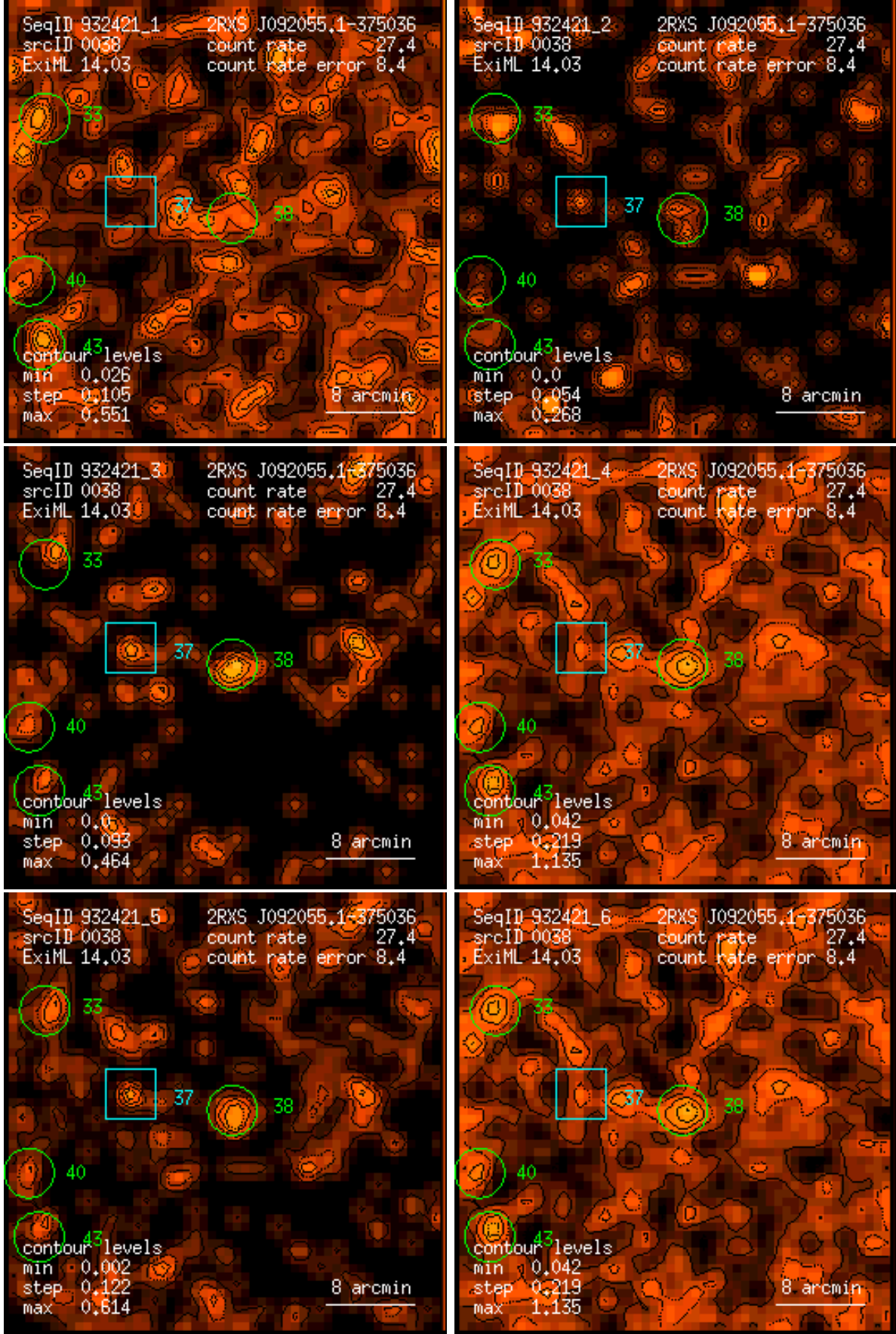
Figure 38: RASS 932421: detection 0038: band rate images, Gaussian filter: (1) PSPC channels 11 – 41, (2) 52 – 90, (3) 91 – 201, (4) 11 – 235, (5) 52 – 201, (6) 11 – 201. Broad band rates in counts/ks. Band rate contour levels in counts/ks/arcmin 2 .
