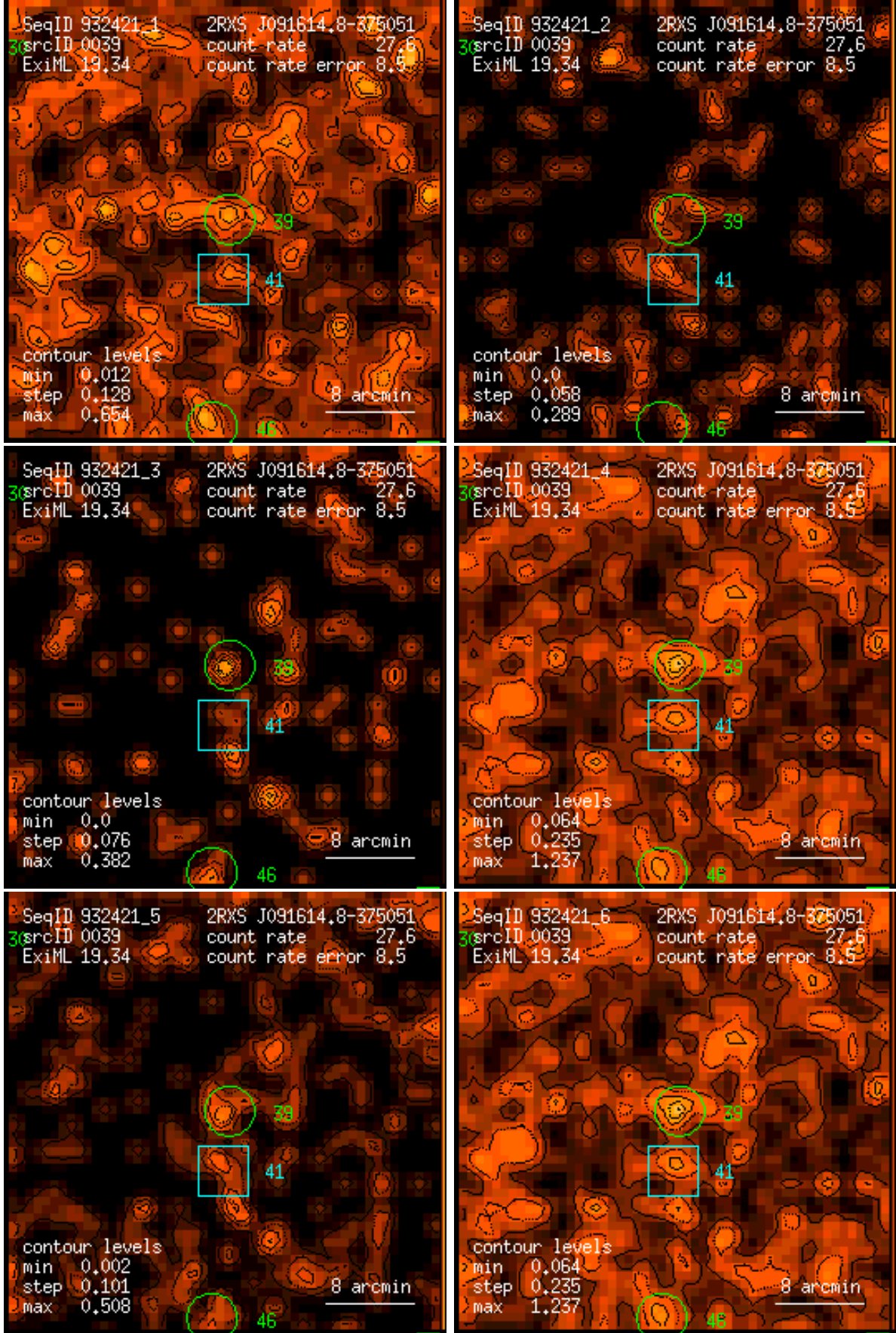
Figure 39: RASS 932421: detection 0039: band rate images, Gaussian filter: (1) PSPC channels 11 – 41, (2) 52 – 90, (3) 91 – 201, (4) 11 – 235, (5) 52 – 201, (6) 11 – 201. Broad band rates in counts/ks. Band rate contour levels in counts/ks/arcmin 2 .
