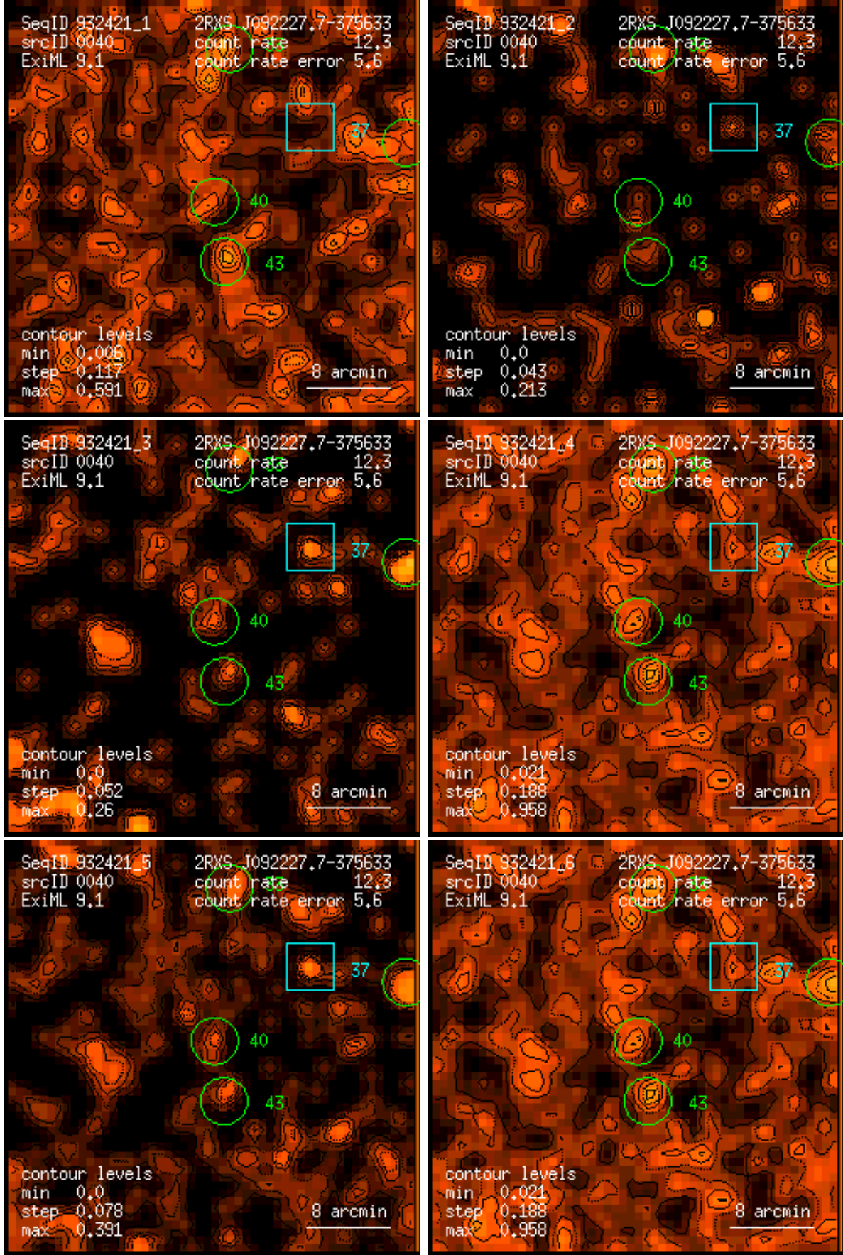
Figure 40: RASS 932421: detection 0040: band rate images, Gaussian filter: (1) PSPC channels 11 – 41, (2) 52 – 90, (3) 91 – 201, (4) 11 – 235, (5) 52 – 201, (6) 11 – 201. Broad band rates in counts/ks. Band rate contour levels in counts/ks/arcmin 2 .
