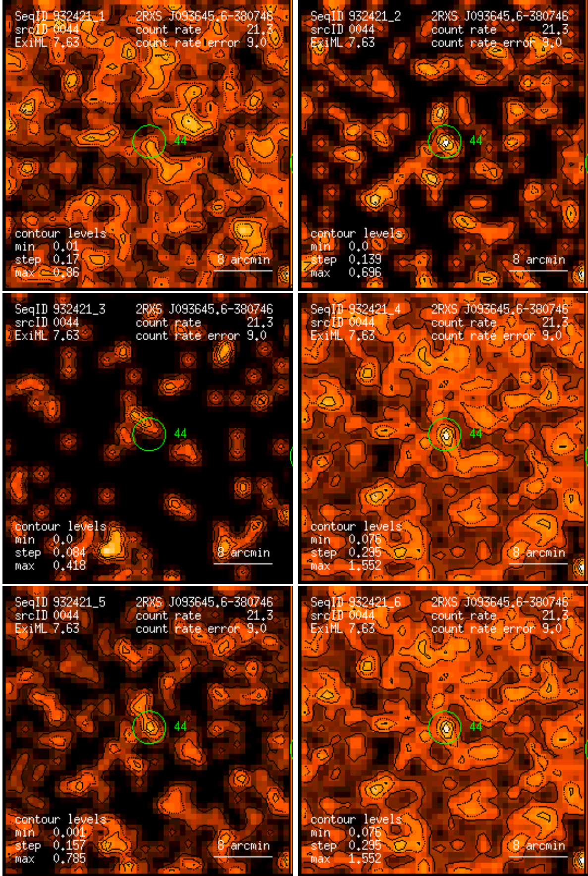
Figure 44: RASS 932421: detection 0044: band rate images, Gaussian filter: (1) PSPC channels 11 – 41, (2) 52 – 90, (3) 91 – 201, (4) 11 – 235, (5) 52 – 201, (6) 11 – 201. Broad band rates in counts/ks. Band rate contour levels in counts/ks/arcmin 2 .
