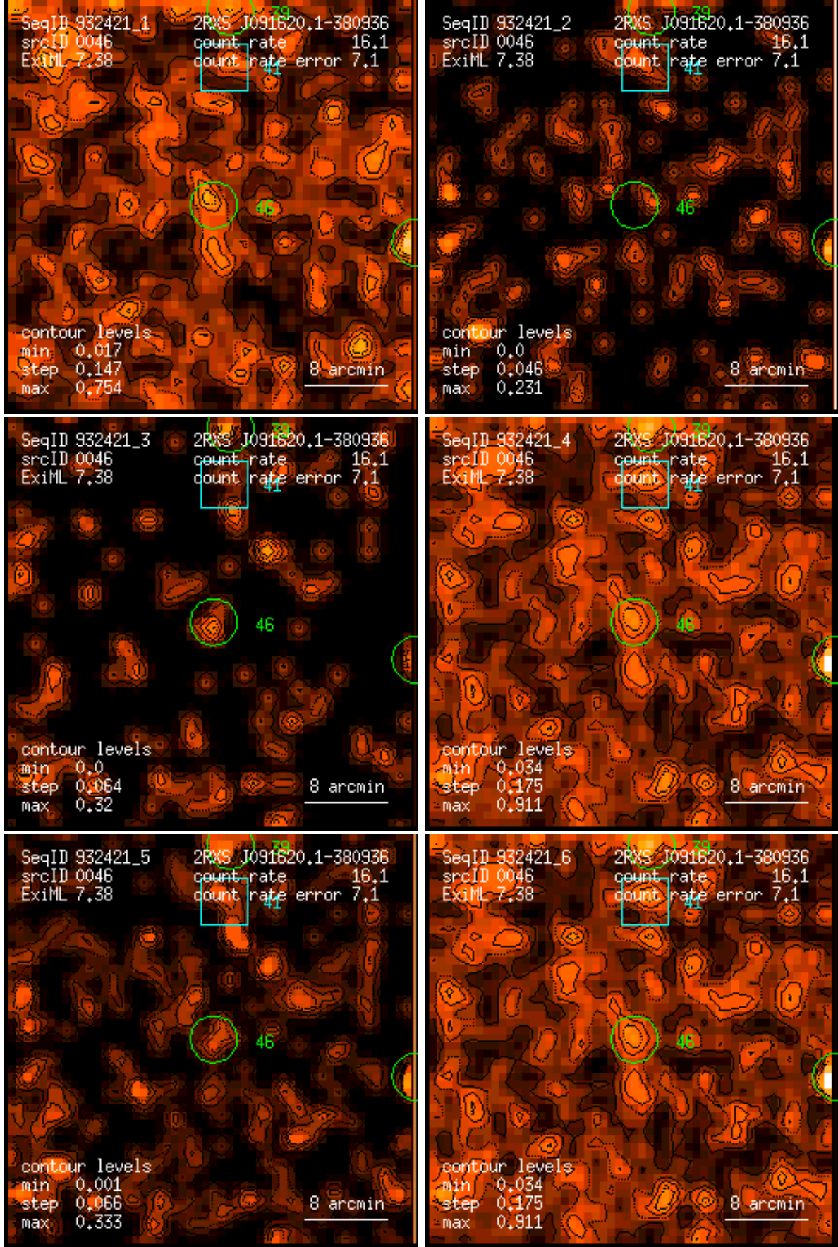
Figure 46: RASS 932421: detection 0046: band rate images, Gaussian filter: (1) PSPC channels 11 – 41, (2) 52 – 90, (3) 91 – 201, (4) 11 – 235, (5) 52 – 201, (6) 11 – 201. Broad band rates in counts/ks. Band rate contour levels in counts/ks/arcmin 2 .
