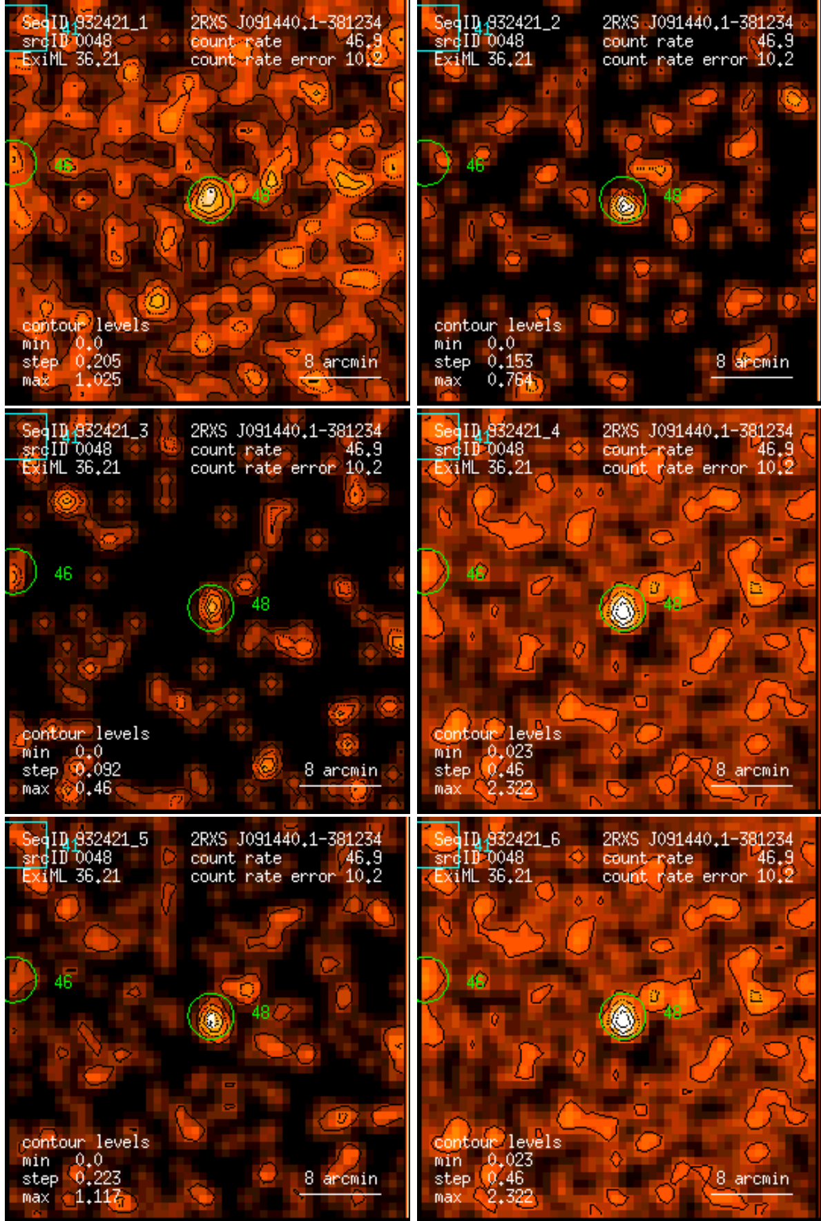
Figure 48: RASS 932421: detection 0048: band rate images, Gaussian filter: (1) PSPC channels 11 – 41, (2) 52 – 90, (3) 91 – 201, (4) 11 – 235, (5) 52 – 201, (6) 11 – 201. Broad band rates in counts/ks. Band rate contour levels in counts/ks/arcmin 2 .
