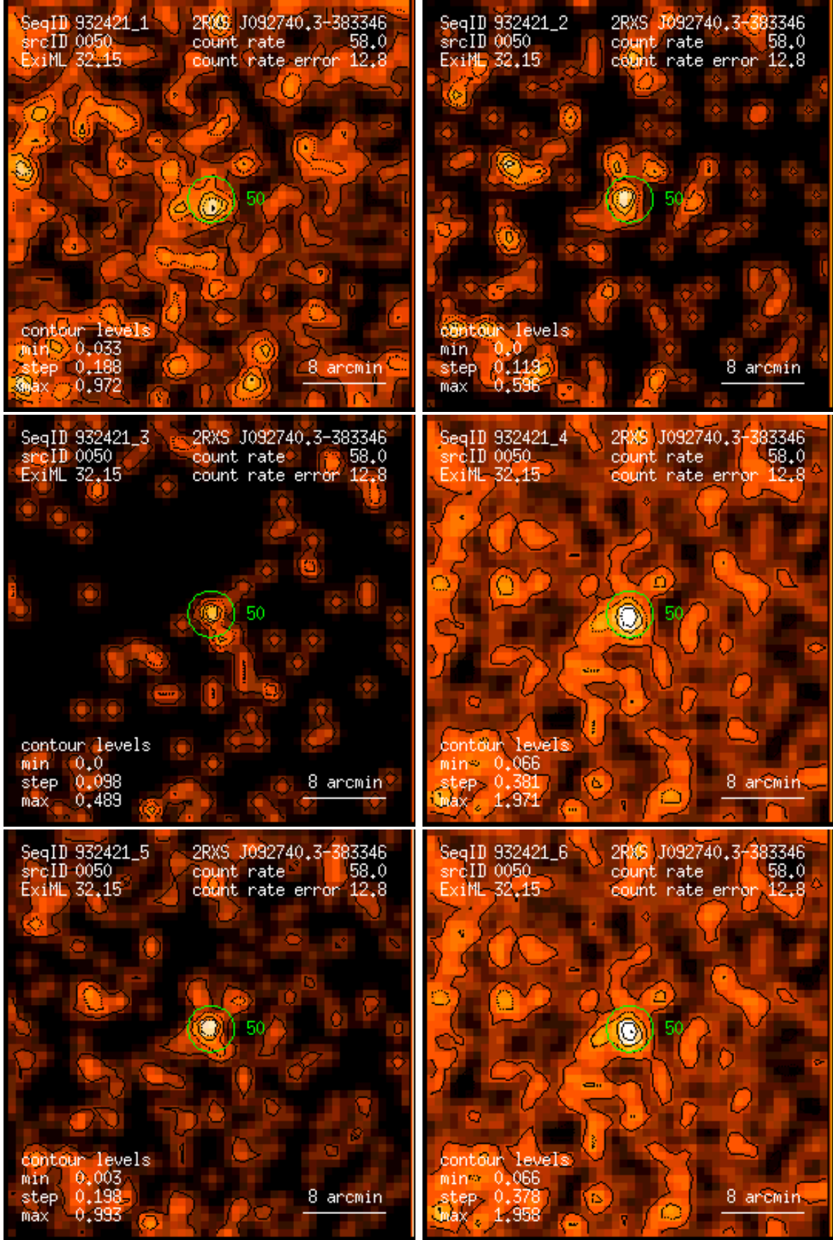
Figure 50: RASS 932421: detection 0050: band rate images, Gaussian filter: (1) PSPC channels 11 – 41, (2) 52 – 90, (3) 91 – 201, (4) 11 – 235, (5) 52 – 201, (6) 11 – 201. Broad band rates in counts/ks. Band rate contour levels in counts/ks/arcmin 2 .
