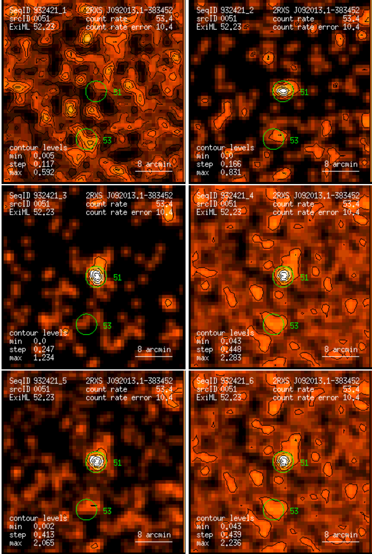
Figure 51: RASS 932421: detection 0051: band rate images, Gaussian filter: (1) PSPC channels 11 – 41, (2) 52 – 90, (3) 91 – 201, (4) 11 – 235, (5) 52 – 201, (6) 11 – 201. Broad band rates in counts/ks. Band rate contour levels in counts/ks/arcmin 2 .
