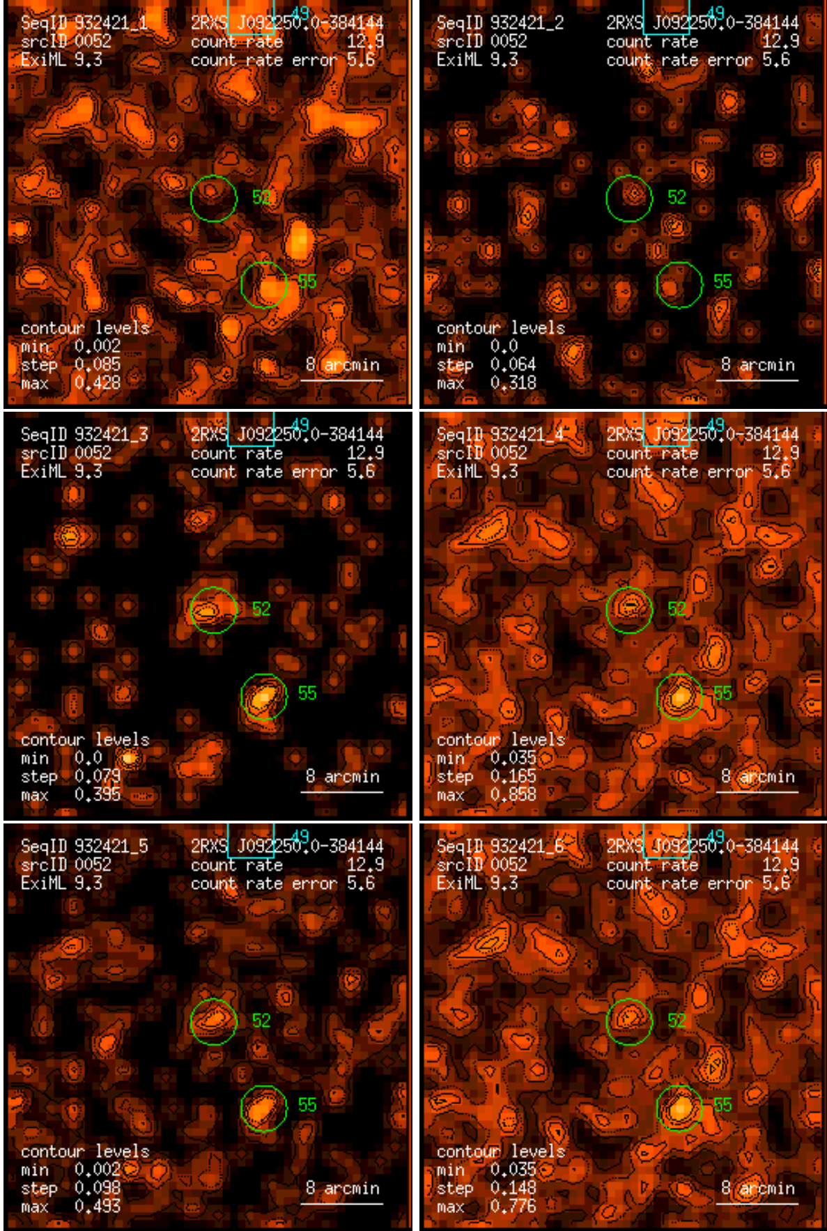
Figure 52: RASS 932421: detection 0052: band rate images, Gaussian filter: (1) PSPC channels 11 – 41, (2) 52 – 90, (3) 91 – 201, (4) 11 – 235, (5) 52 – 201, (6) 11 – 201. Broad band rates in counts/ks. Band rate contour levels in counts/ks/arcmin 2 .
